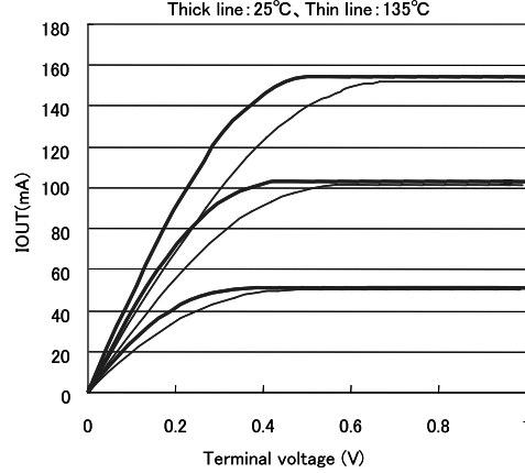
Fig.8 IOU(B) vs. Terminal voltage
