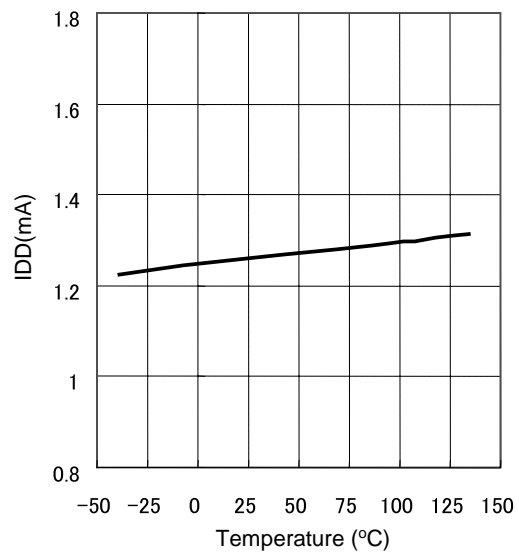
Fig.6 IDD vs. temperature
