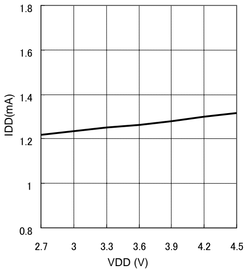
Fig.5 IDD vs. VDD
