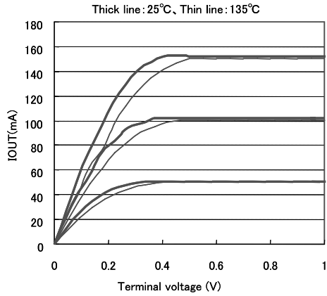
Fig.9 IOU(G) vs. Terminal voltage
