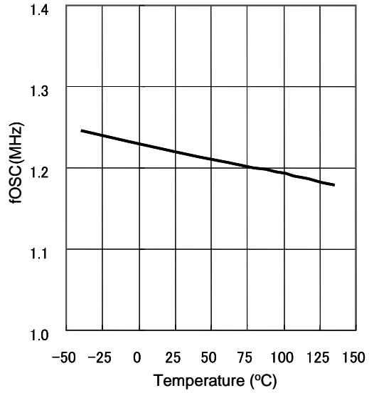
Fig.4 fOSC vs. temperature
