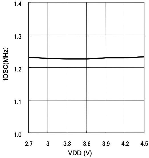
Fig.3 fOSC vs. VDD
