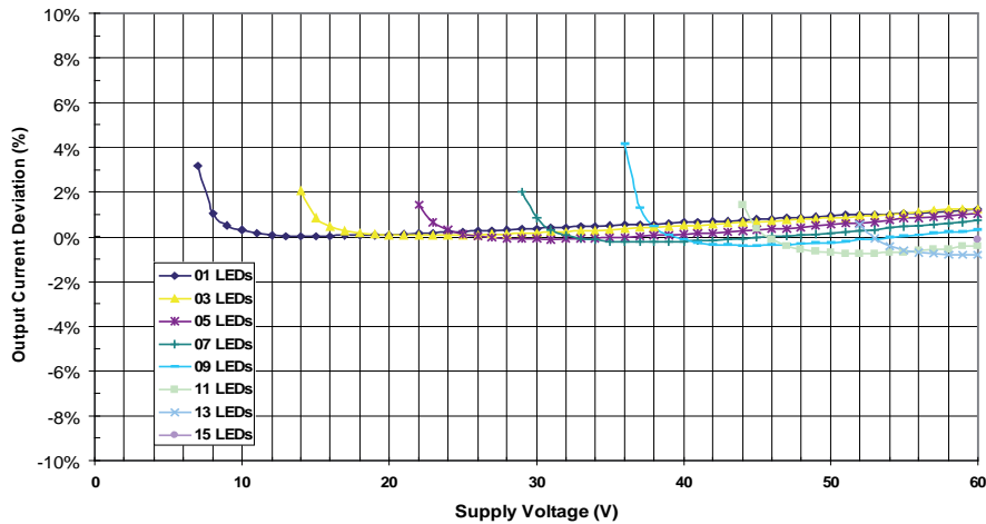
ZXLD1366 Output Current Deviation L=220μH
