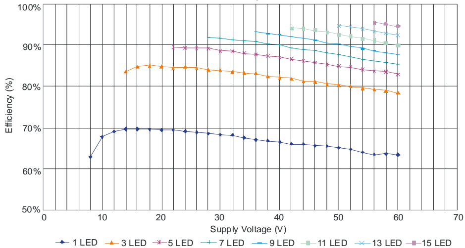
ZXLD1362 Efficiency L = 68 \mu H
