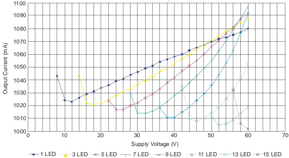
ZXLD1362 Output Current L = 68 \mu H
