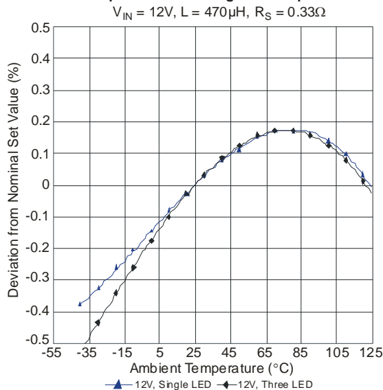
Output Current Change vs. Temperature V IN = 12V, L = 470µH, R S = 0.33Ω
