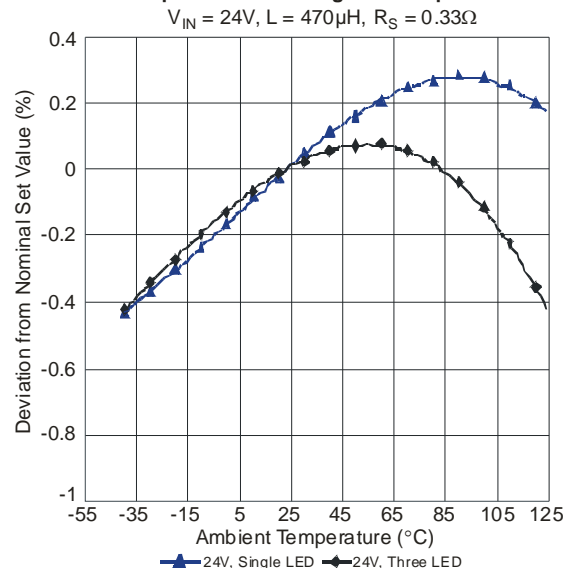
Output Current Change vs. Temperature V IN = 24V, L = 470µH, R S = 0.33Ω
