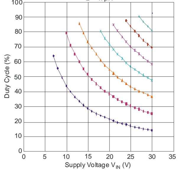
ZXLD1360 Duty Cycle L = 47µH
