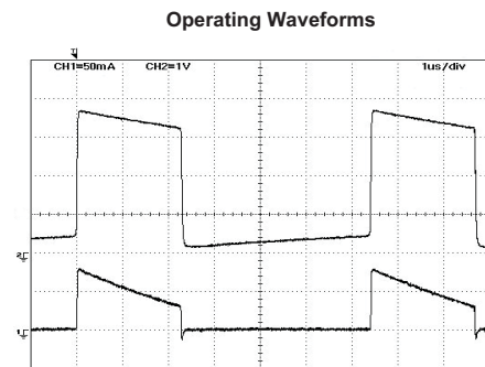
Channel 1 (lower): LED current I_{Led} . 50mA/div. Channel 2 (upper): Voltage at Vout pin. 1V/div
