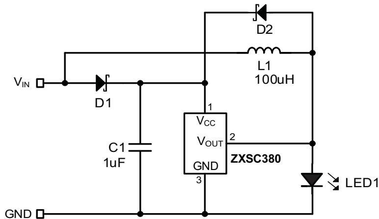
Figure 5 ZXSC380 in bootstrap mode
