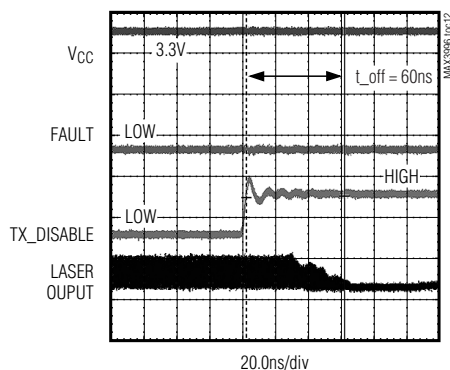
TRANSMITTER DISABLE
