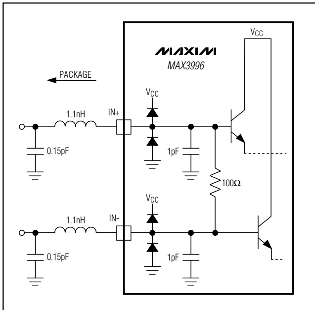
Figure 16. Data Inputs
