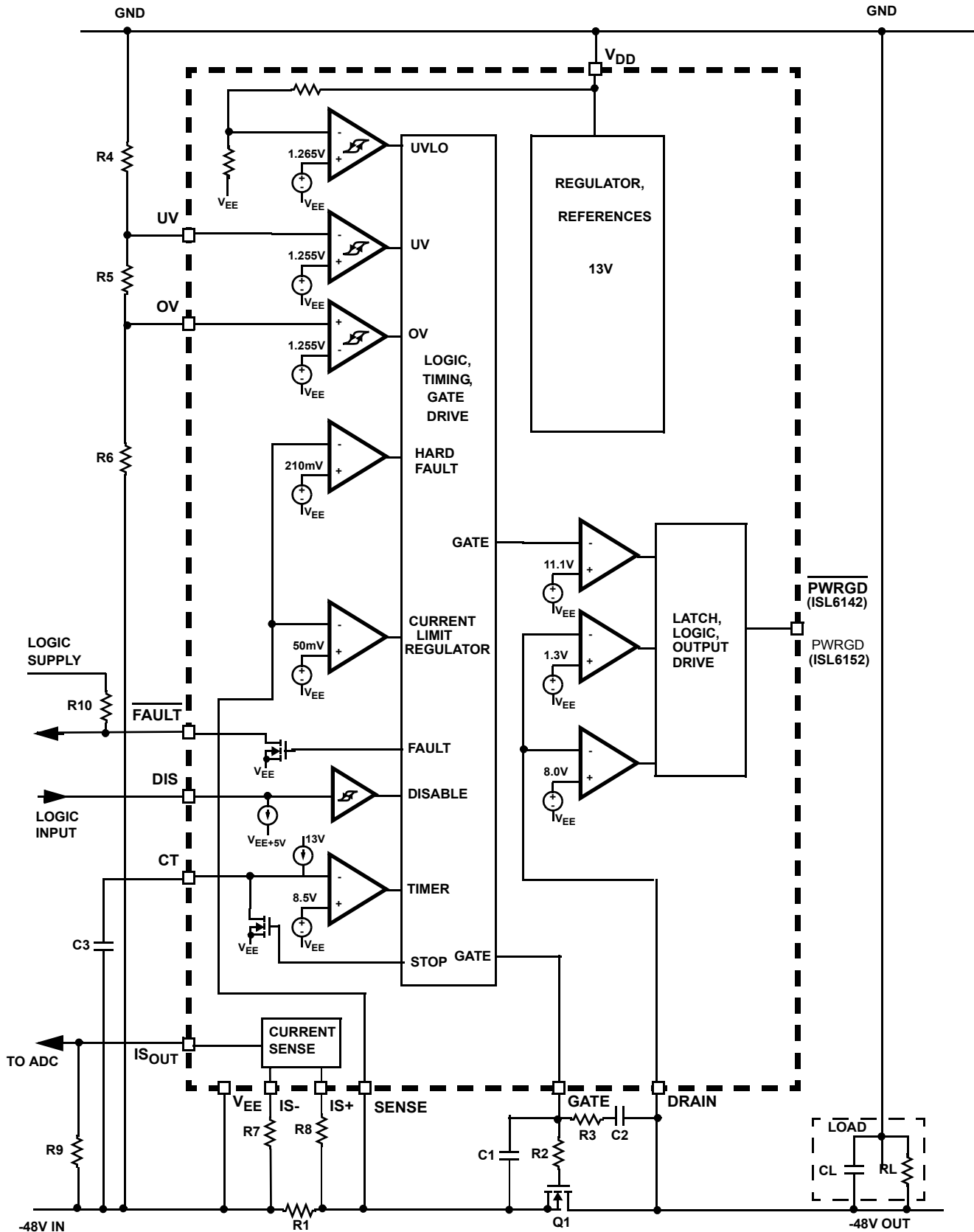
FIGURE 1. BLOCK DIAGRAM
