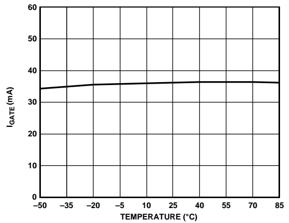
Figure 13. I_{GATE} (FCL, Sink) vs. Temperature ( V_{GATE} = 2 V )
