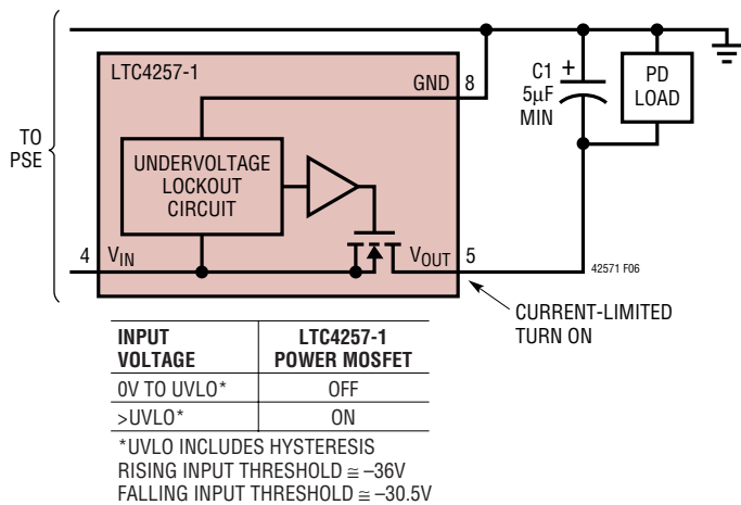
Figure 6. LTC4257-1 Undervoltage Lockout
