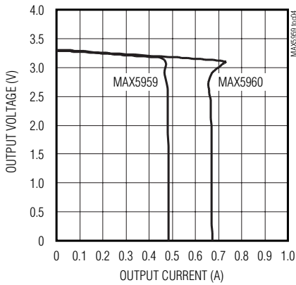
3.3VAUXO_ OUTPUT VOLTAGE vs. OUTPUT CURRENT
