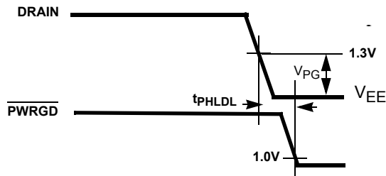
FIGURE 4A. DRAIN TO \overline{\text{PWRGD}} TIMING (ISL6141)
