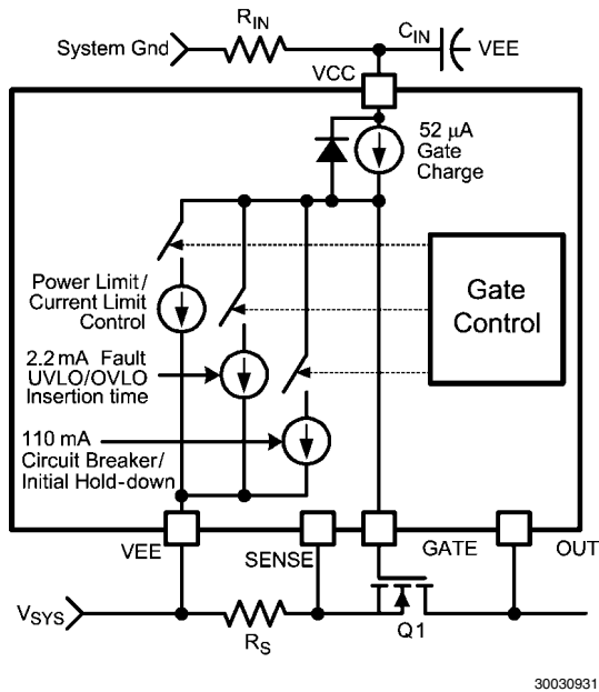
FIGURE 4. Gate Control
