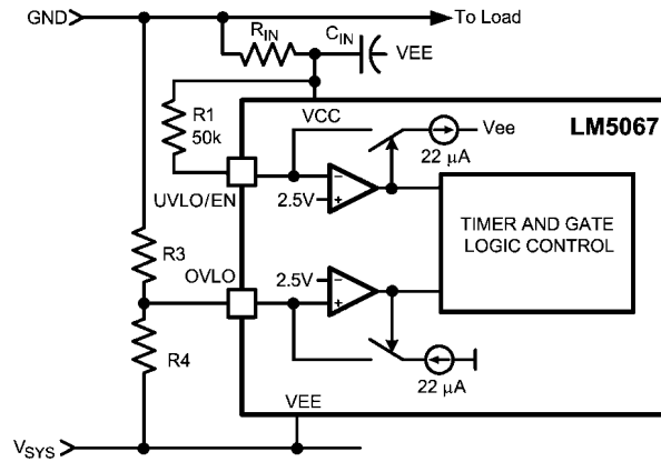
FIGURE 13. UVLO = POR_{EN}
