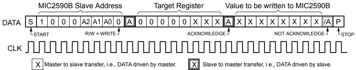
Figure 8. WRITE_BYTE Protocol
