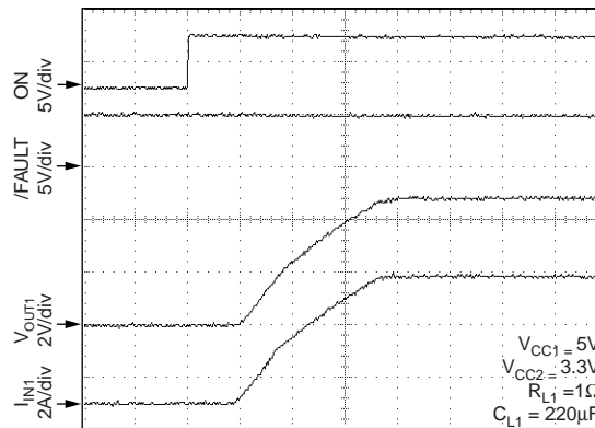
Turn-On (Channel 1)
