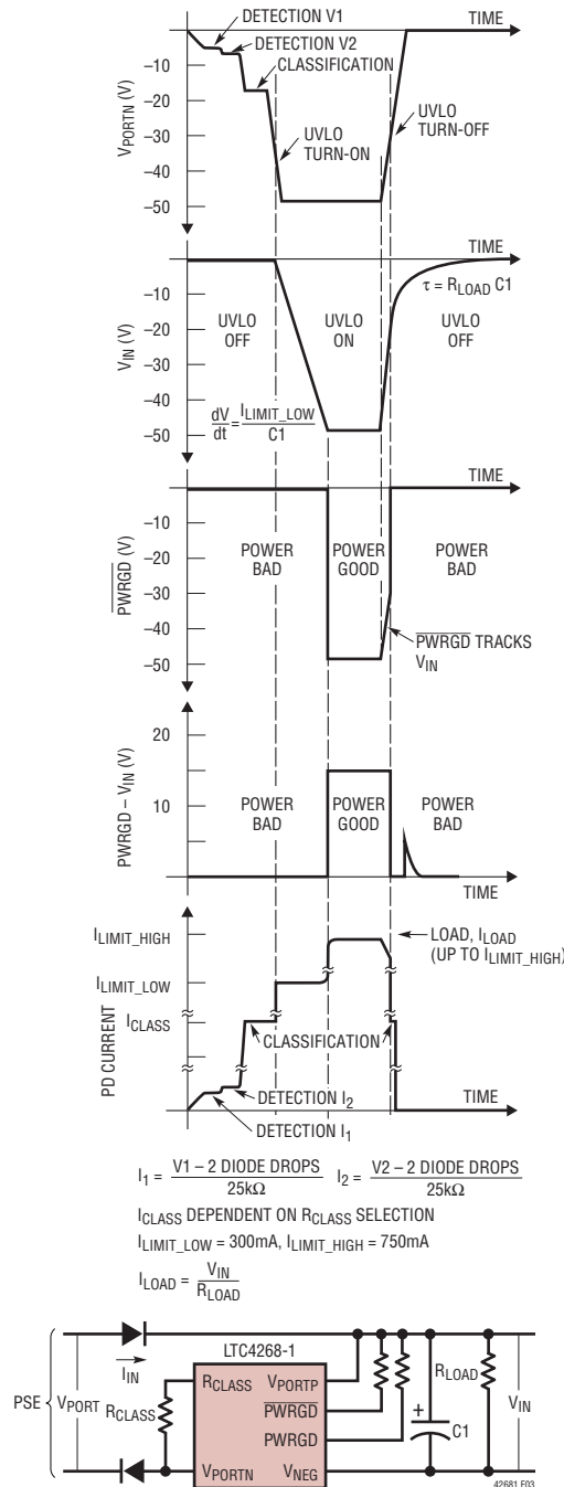
Figure 3. V_{IN} Voltage, \overline{PWRGD} , \overline{PWRGD} - V_{IN} and PD Current as a Function of Port Voltage
