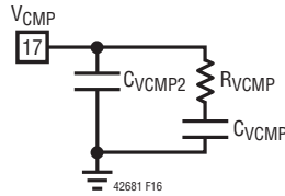
Figure 16. V_{C_{MP}} Compensation Network
