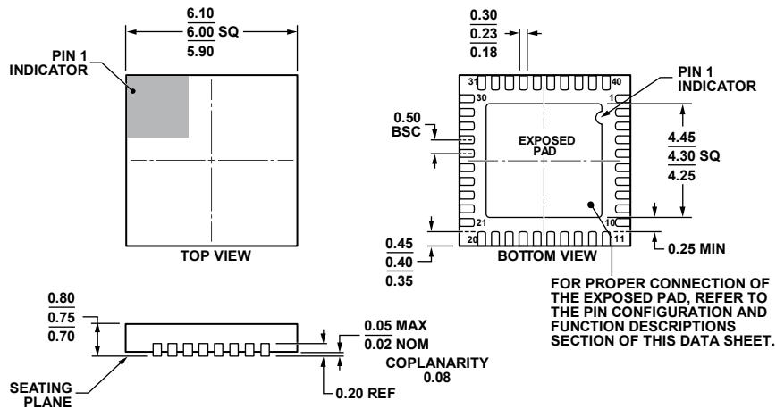
COMPLIANT TO JEDEC STANDARDS MO-220-WJJD. Figure 90. 40-Lead Lead Frame Chip Scale Package [LFCSP_WQ] 6 mm x 6 mm Body, Very Very Thin Quad (CP-40-10) Dimensions shown in millimeters
