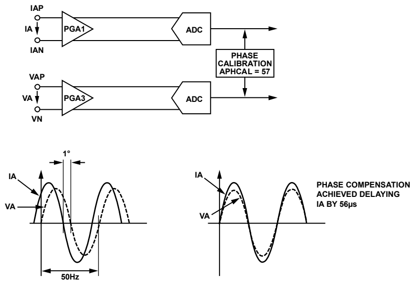
Figure 53. Phase Calibration on Voltage Channels
