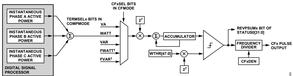
Figure 70. Energy-to-Frequency Conversion
