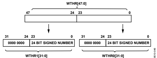
Figure 64. WTHR[47:0] Communicated As Two 32-Bit Registers
