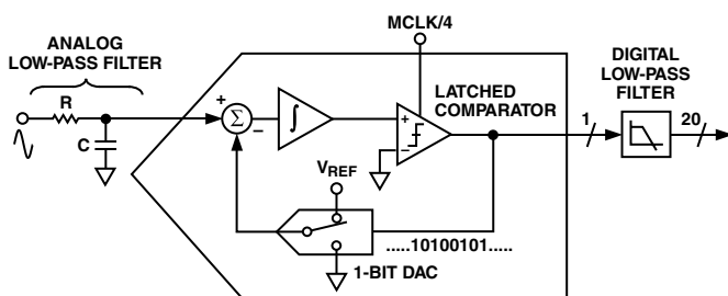
Figure 19. First Order Sigma-Delta ( \Sigma - \Delta ) ADC
