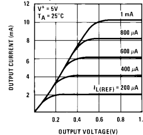
Output Characteristics
