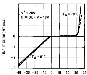
Input Current Beyond Signal Range (Pin 5)
