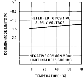
Common-Mode Limits
