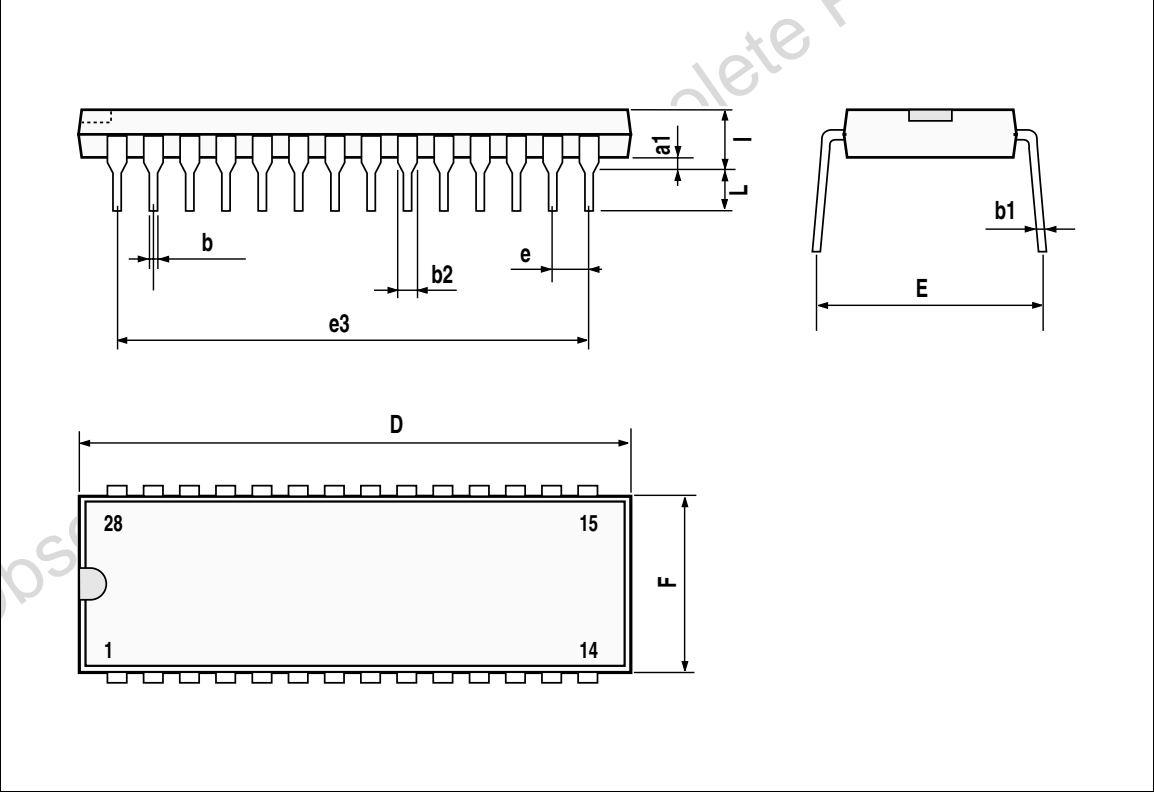
Figure 10. PDIP28 - Package Dimensions
