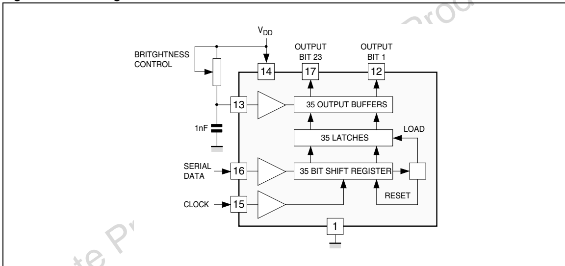
Figure 3. Block Diagram
