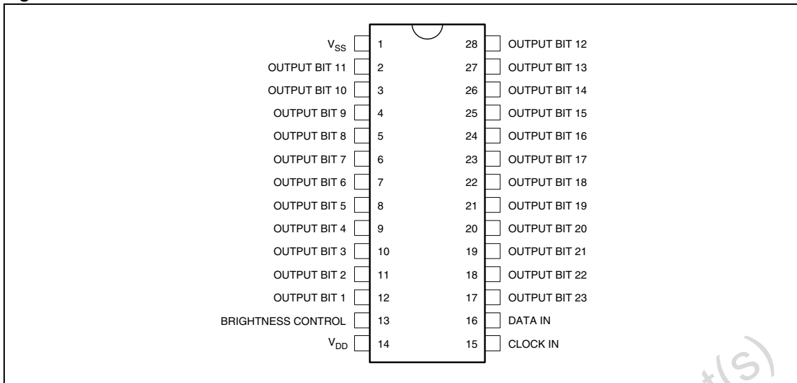
Figure 2. Pin Connections
