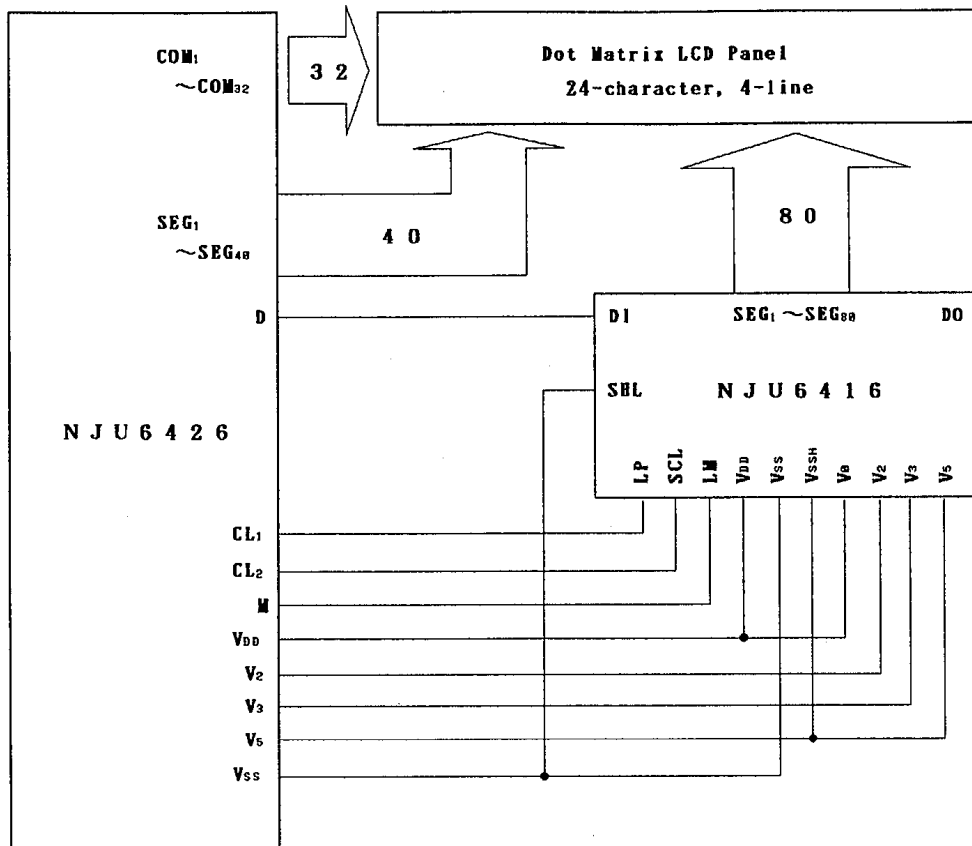
24-character 4-line Display Example (NJU6426 + NJU6416)
