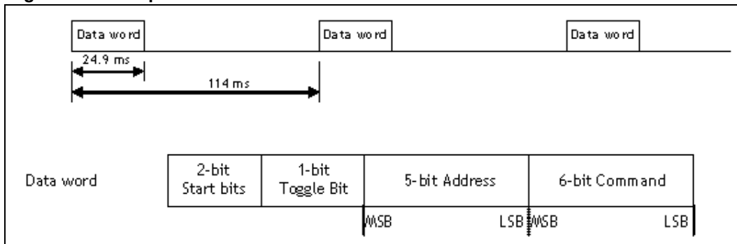
Figure 23. RC-5 reception example
