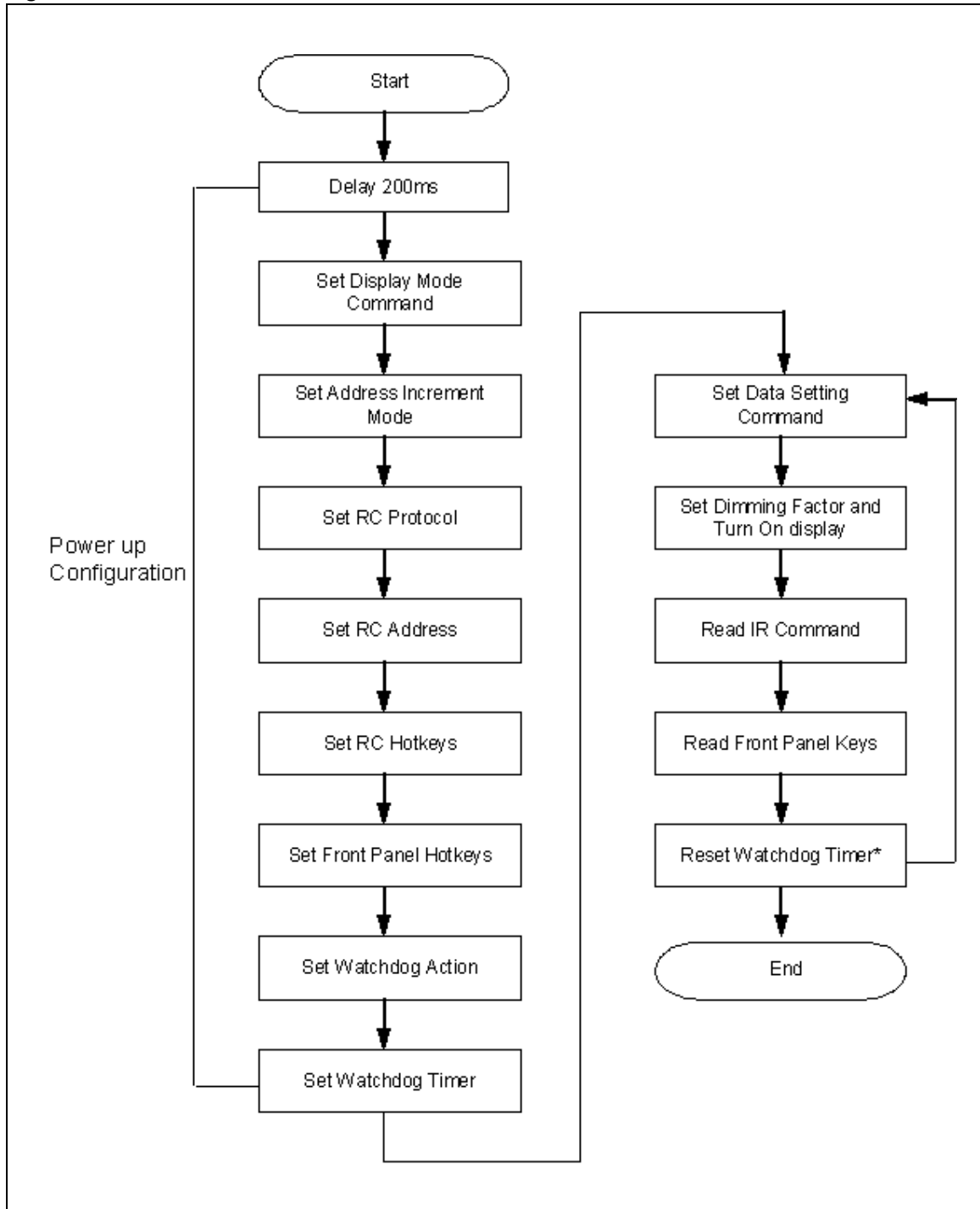
Figure 20. Recommended software flow
