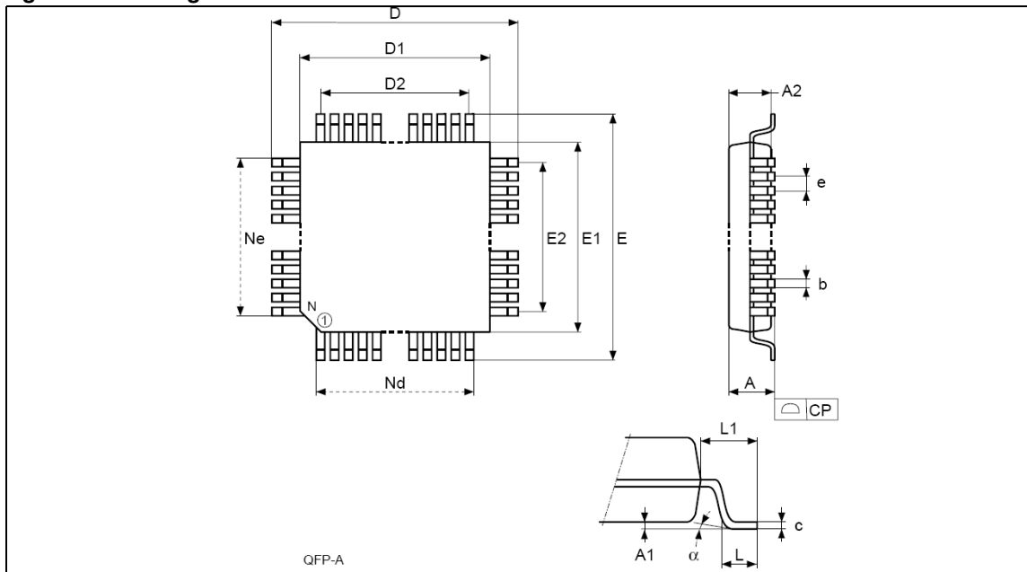
Figure 34. Package dimensions
