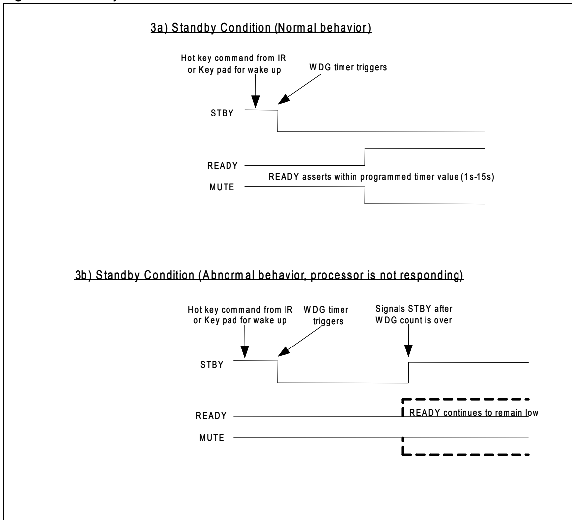
Figure 5. Standby condition
