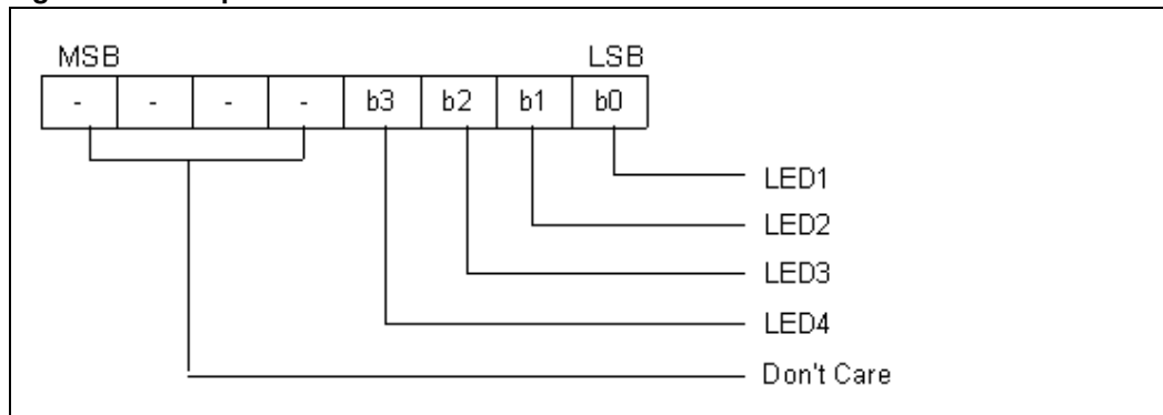
Figure 12. LED port data WRITE command order
