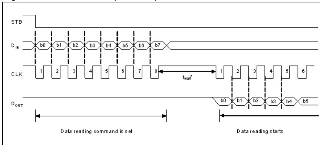
Figure 29. Data transmission (data READ)
