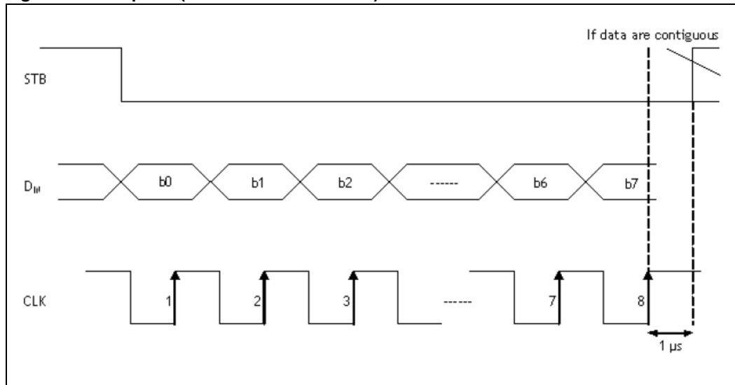
Figure 29. Data transmission (data READ)
