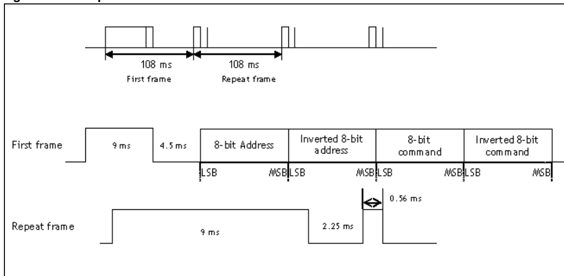
Figure 26. NEC protocol transmission waveforms
