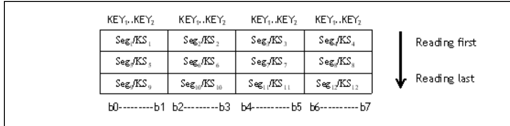
Figure 11. Key storage and READ access
