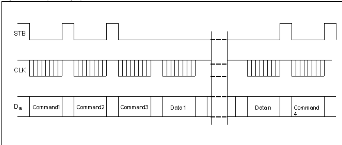
Figure 32. Updating specific address
