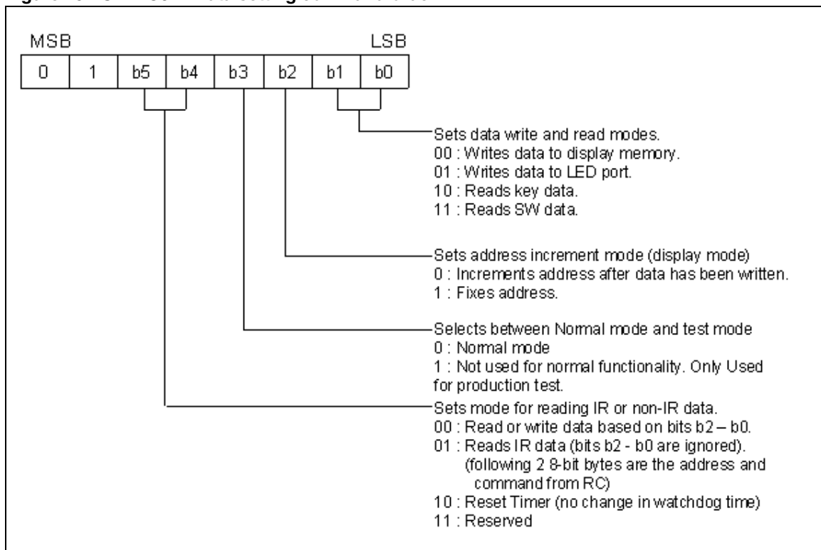
Figure 15. STFPC311 Data setting command order
