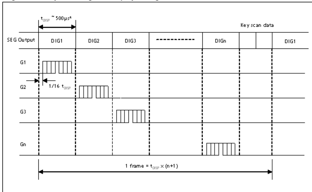
Figure 27. Key scanning and display timing
