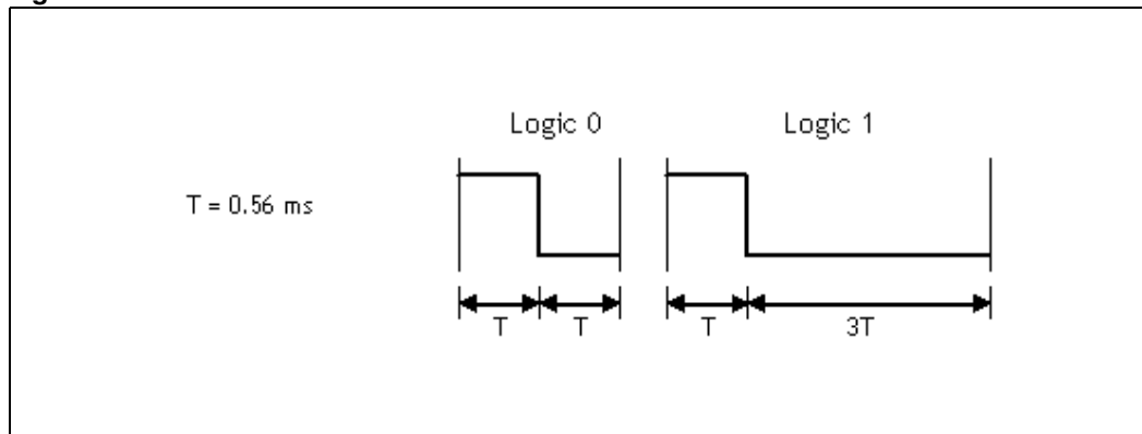
Figure 25. Pulse distance modulation.
