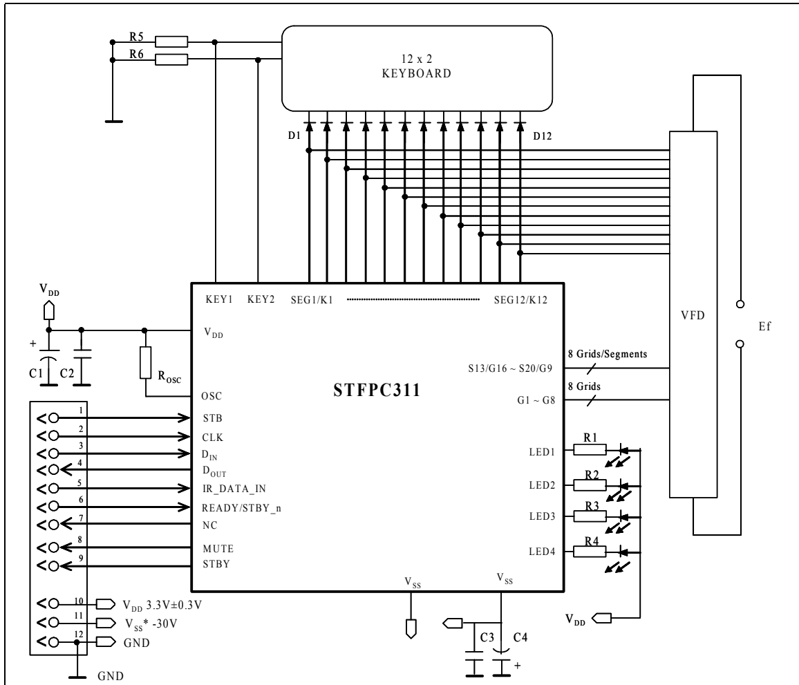
Figure 33. Typical application circuit
