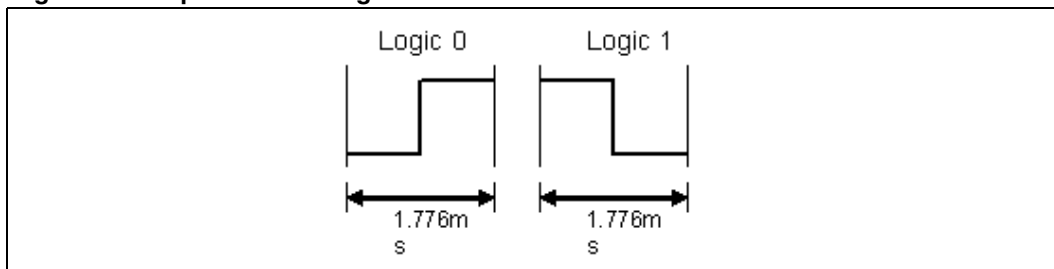
Figure 22. RC-5 protocol frame
