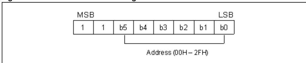
Figure 16. STFPC311 Address Setting Command Order
