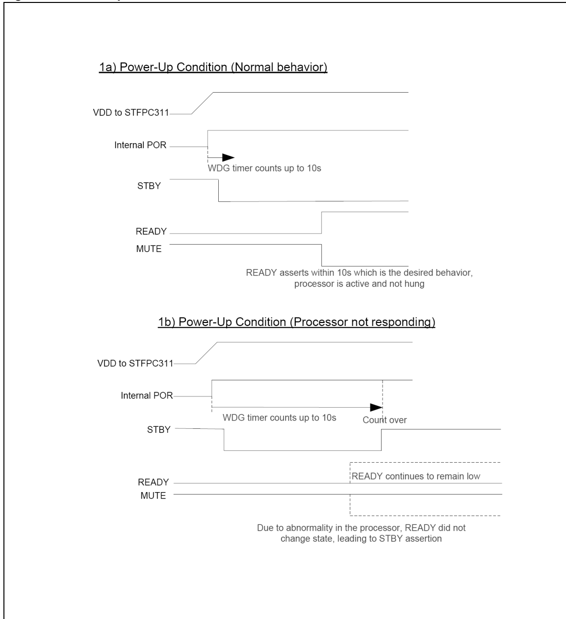
Figure 3. Power-up condition
