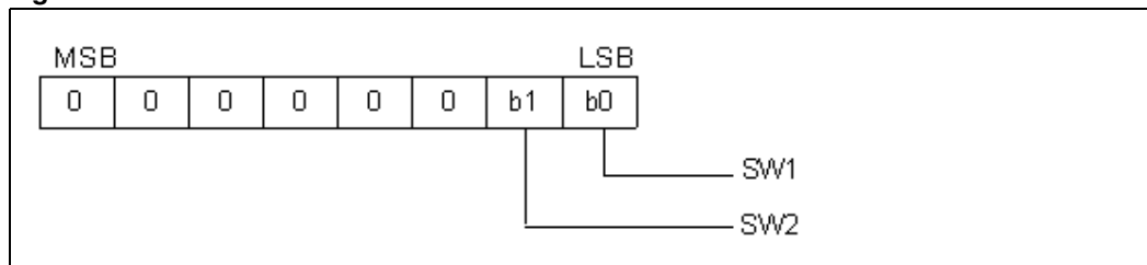
Figure 13. SW data READ Command order
