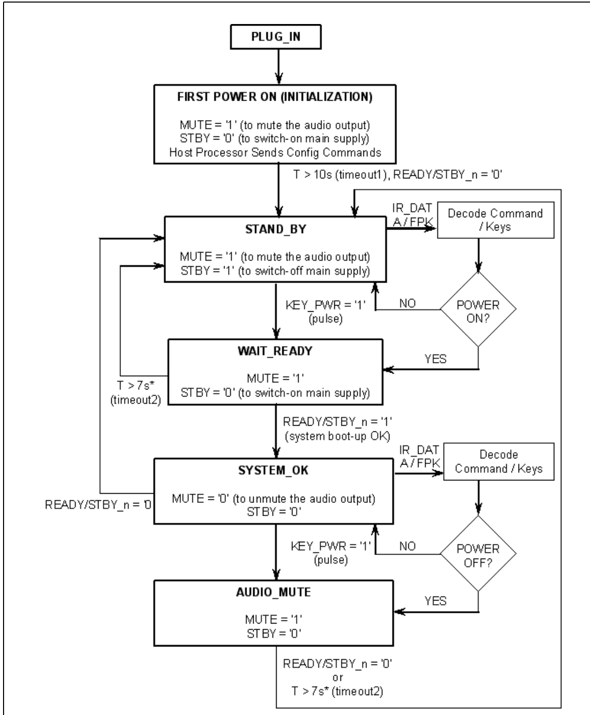
Figure 6. Timing power standby sequencer flow chart
