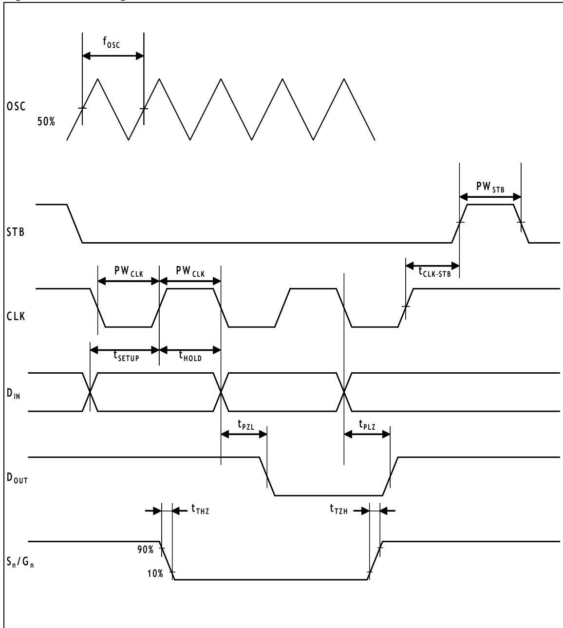
Figure 30. Switching characteristic waveforms
