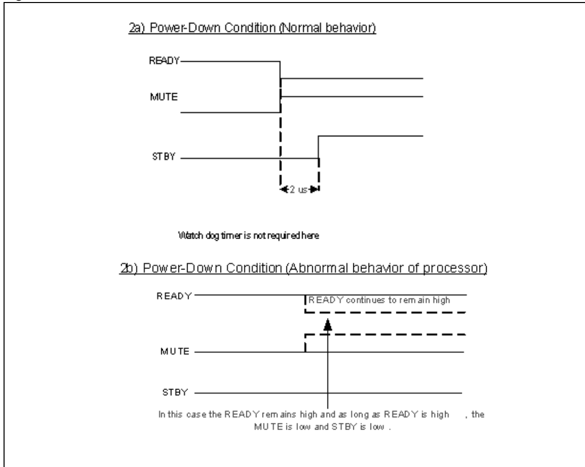
Figure 4. Power-down condition
