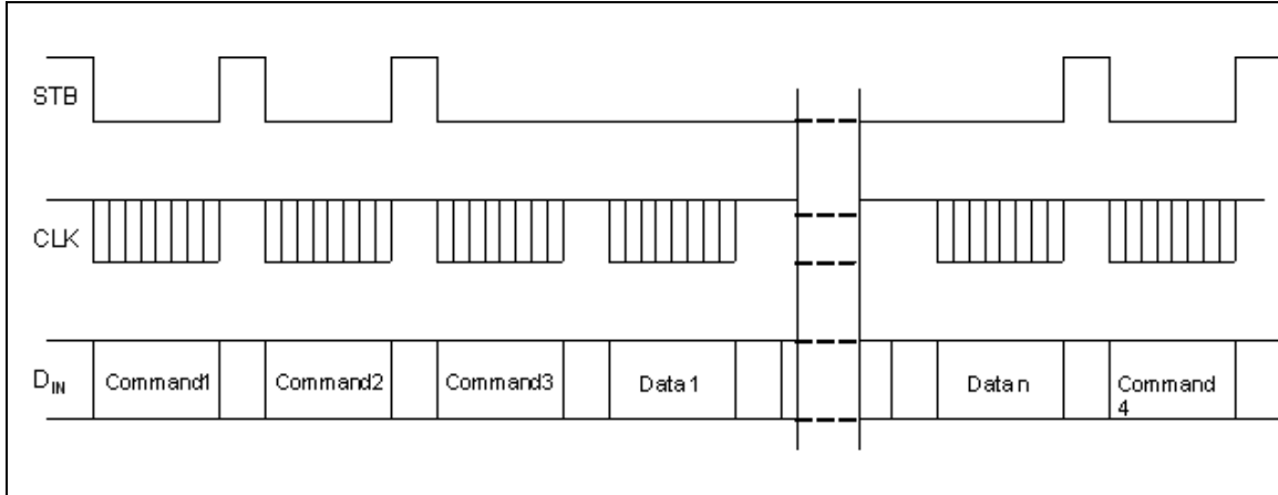
Figure 31. Updating display memory by incrementing address
