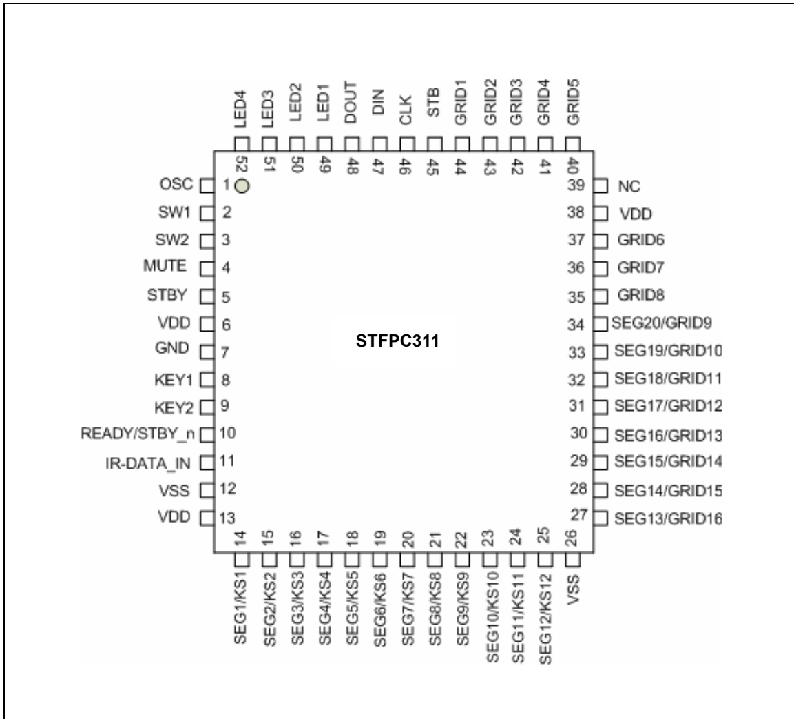
Figure 2. Connection diagram (top view PQFP-52)
