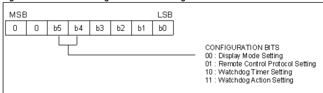
Figure 14. STFPC311 Configuration mode setting command order
