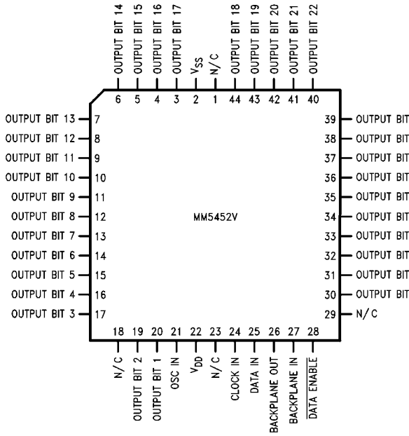
Top View Order Number MM5452V See NS Package Number V44A
