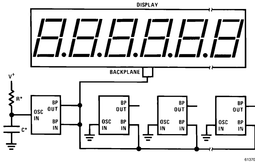
FIGURE 5. Parallel Backplane Outputs
