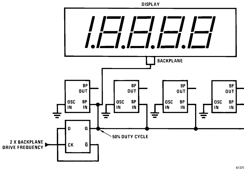
FIGURE 6. External Backplane Clock
