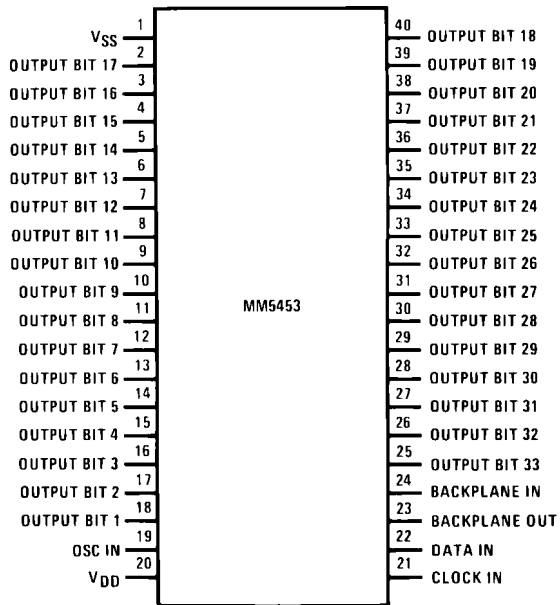
Top View Order Number MM5453N See NS Package Number N40A
