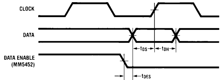
FIGURE 2. Timing Diagram
