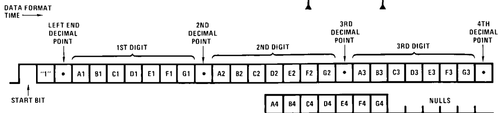
FIGURE 4. Typical 4 1/2-Digit Display Application
