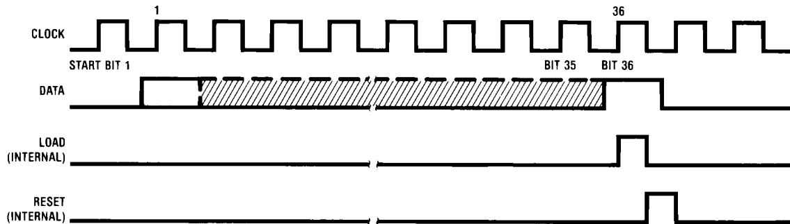
FIGURE 3. Input Data Format
