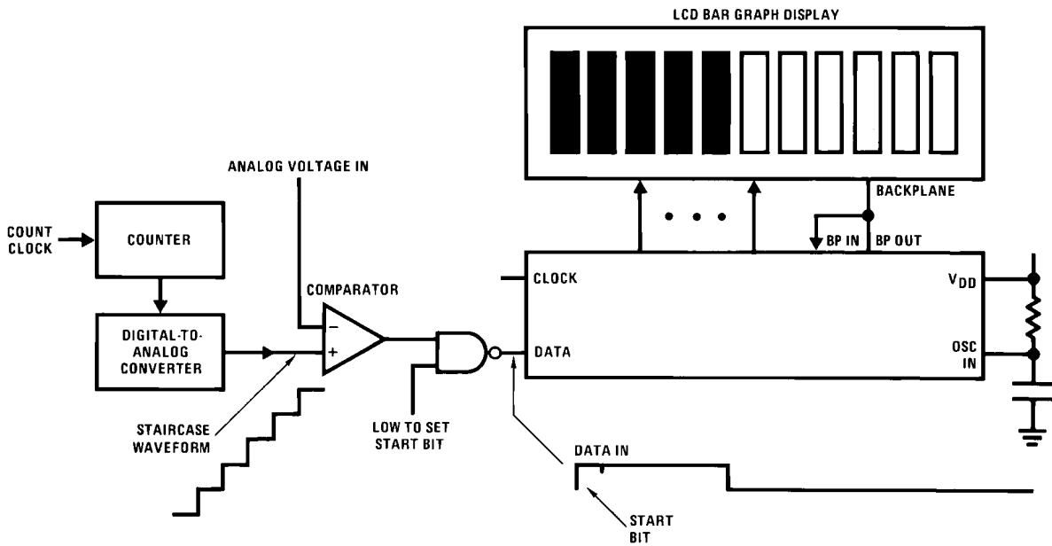
FIGURE 8. Analog Display
