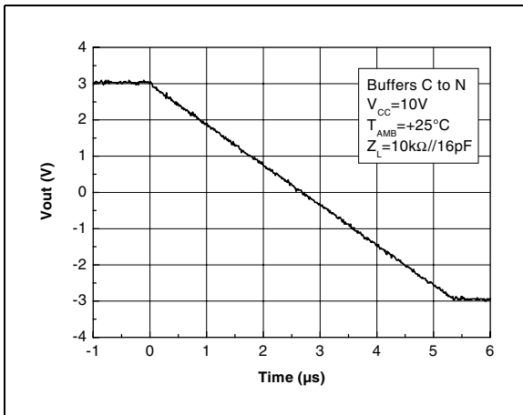
Figure 30. Large signal response - buffers C to N
