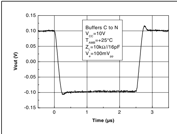
Figure 34. Small signal response - buffers C to N
