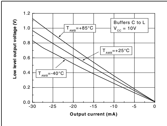
Figure 16. Voltage output low ( V_{OL} ) vs. output current - Buffers C to L
