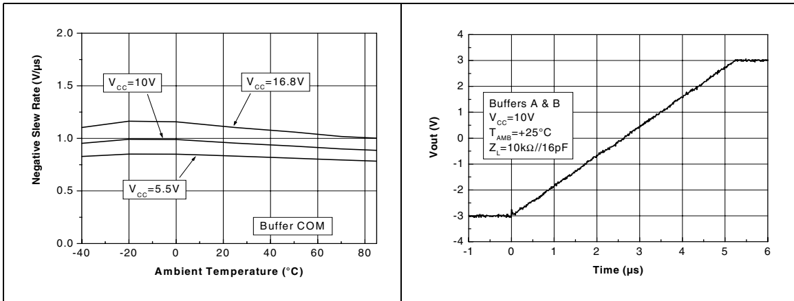
Figure 28. Large signal response - buffers A & B
