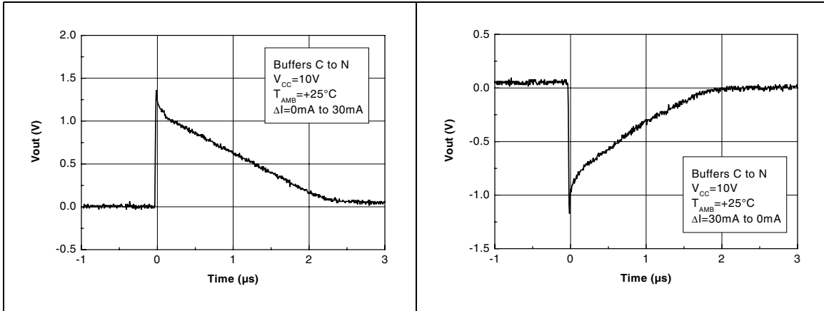
Figure 38. Output voltage response to current transient - buffers C to N Figure 39. Output voltage response to current transient - buffers C to N
