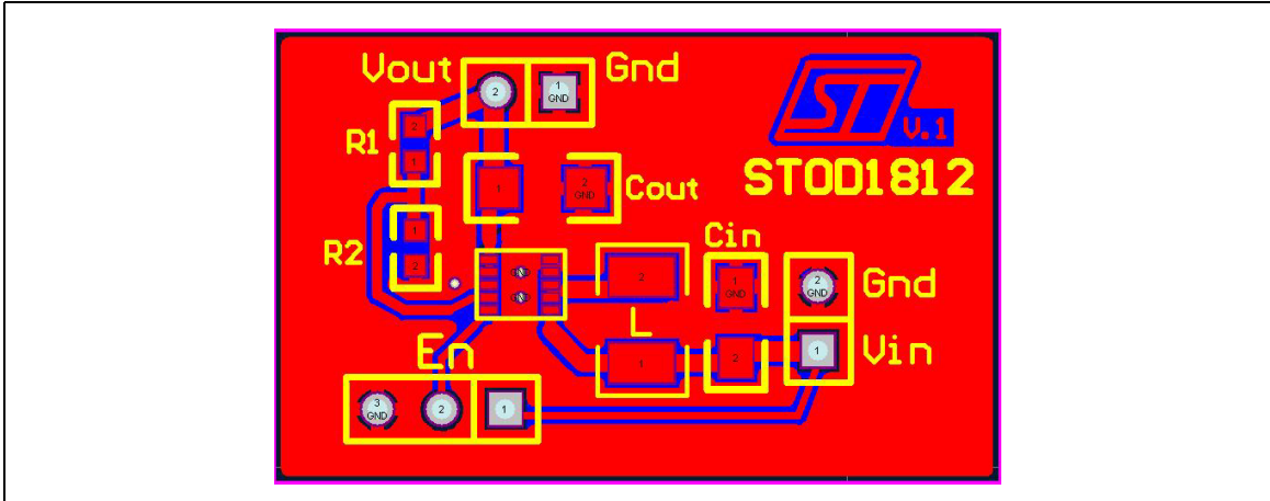
Figure 6. Suggested demonstration board schematic (top layer view)
