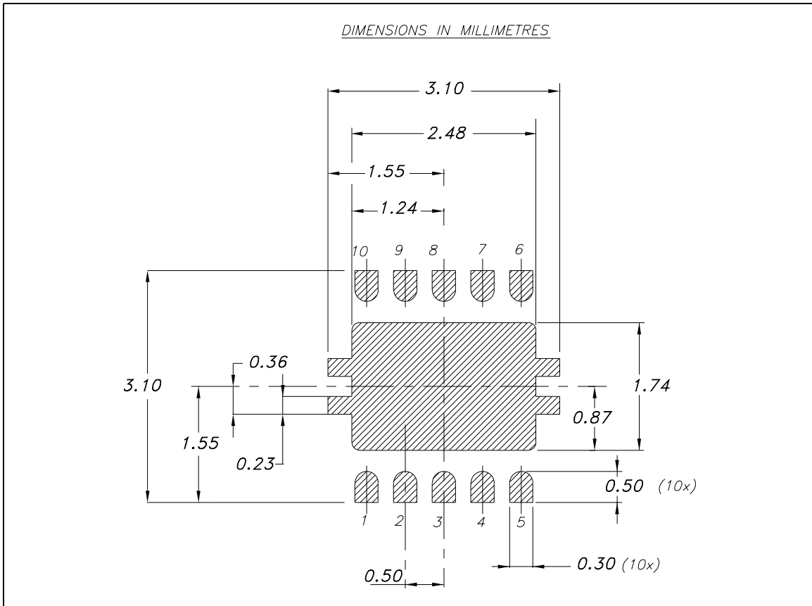
Figure 16. DFN10L footprint - recommended data
