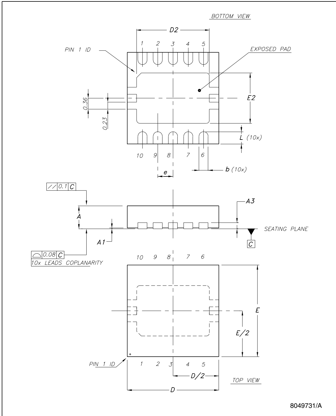
Figure 15. DFN10L package outline
