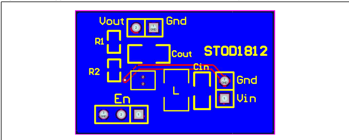
Figure 7. Suggested demonstration board schematic (bottom layer view)
