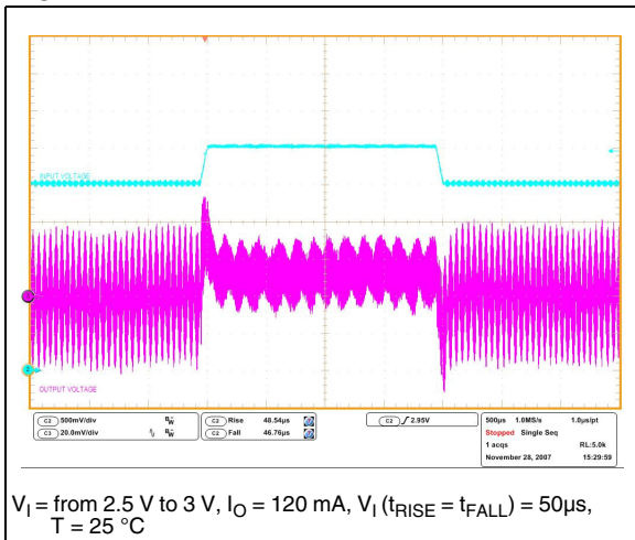
Figure 12. Line transient
