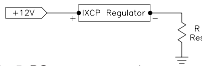
Fig. 5. DC surge suppression
