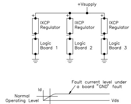
Fig.8. Low cost current regulators instead of fuses
