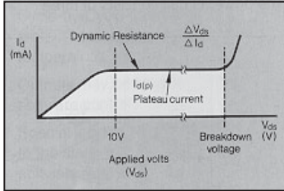
Fig. 1. Current Regulator Output Characteristics
