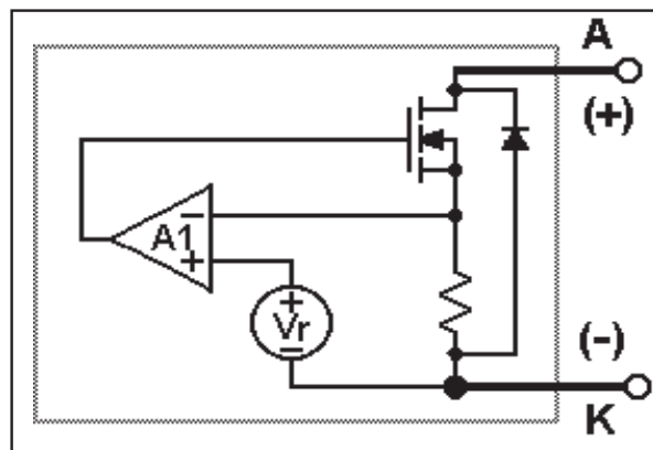
Fig. 2. Block diagram for the non-switchable regulator
