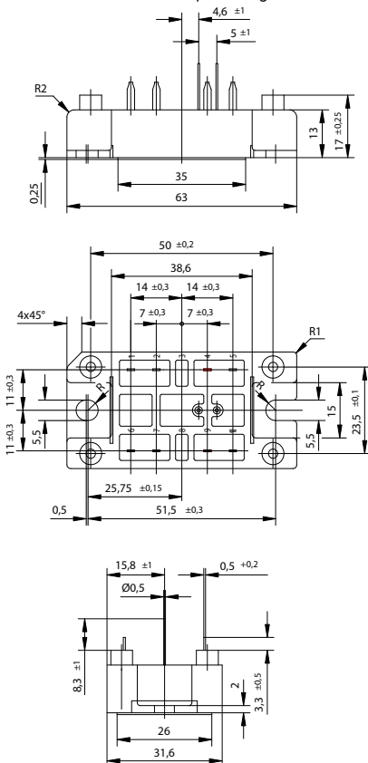
X103 V1-A-Pack See data sheet for pin arrangement
