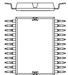
GMM 3x xxx - SMD IPC 75PX330GD SURFACE MOUNT DEVICE
