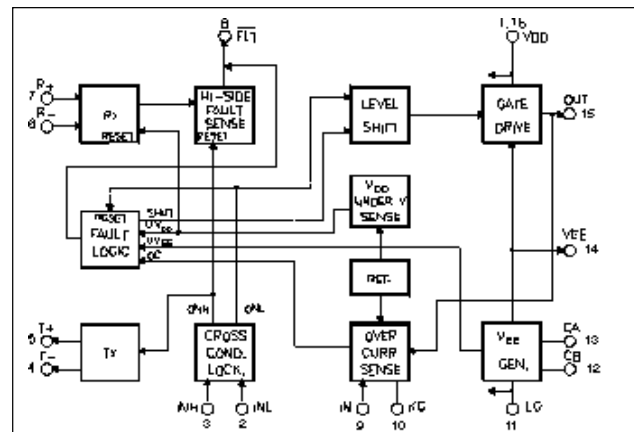
Block diagram IXBD4410
