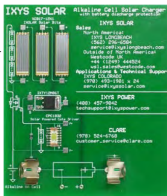
Solar Charger reference design for AA batteries
