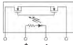
Block diagram CPC1219Y
