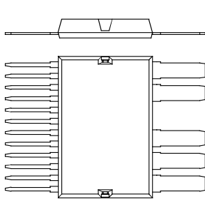
GWM xxx - SL STRAIGHT LEADS
