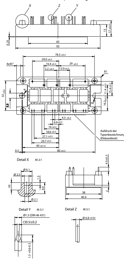
X104 V2-Pack See data sheet for pin arrangement
