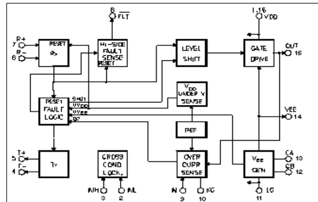
Block diagram IXBD 4411
