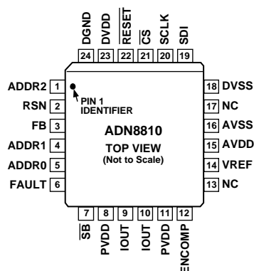
Figure 3. Pin Configuration
