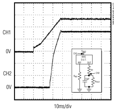
STARTUP DELAY ( V_{BIAS} = 2.7\text{V} , I_{REF} = 2.5\text{mA} )
