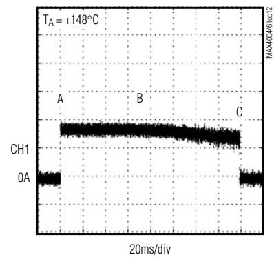
SHORT-CIRCUIT RESPONSE ( V_{BIAS} = 5\text{V} )
