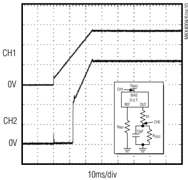
STARTUP DELAY ( V_{BIAS} = 2.7\text{V} , I_{REF} = 250\text{nA} )
