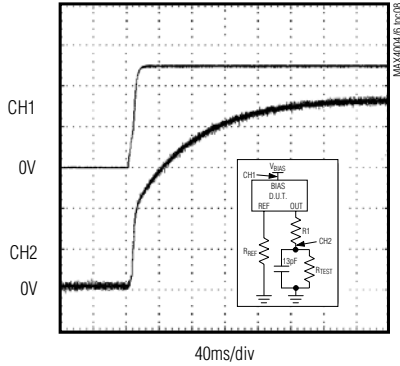
STARTUP DELAY ( V_{BIAS} = 5\text{V} , I_{REF} = 250\text{nA} )
