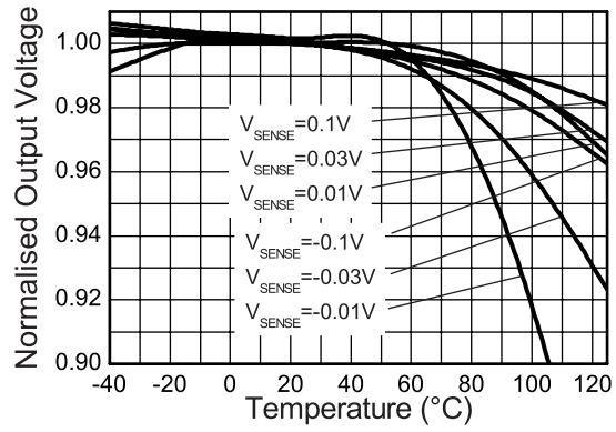
Output v Temperature
