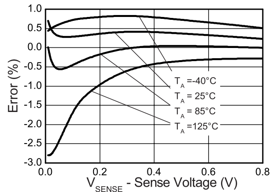
Error v Forward Sense Voltage
