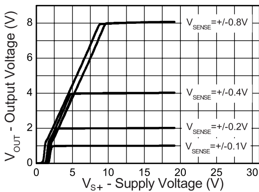
Output v Supply Voltage
