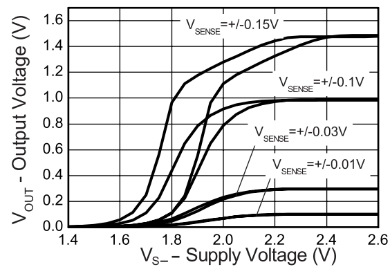
Output v Supply Voltage
