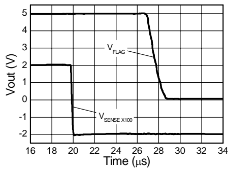
Small Sig Zero Crossing Response
