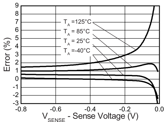
Error v Reverse Sense Voltage
