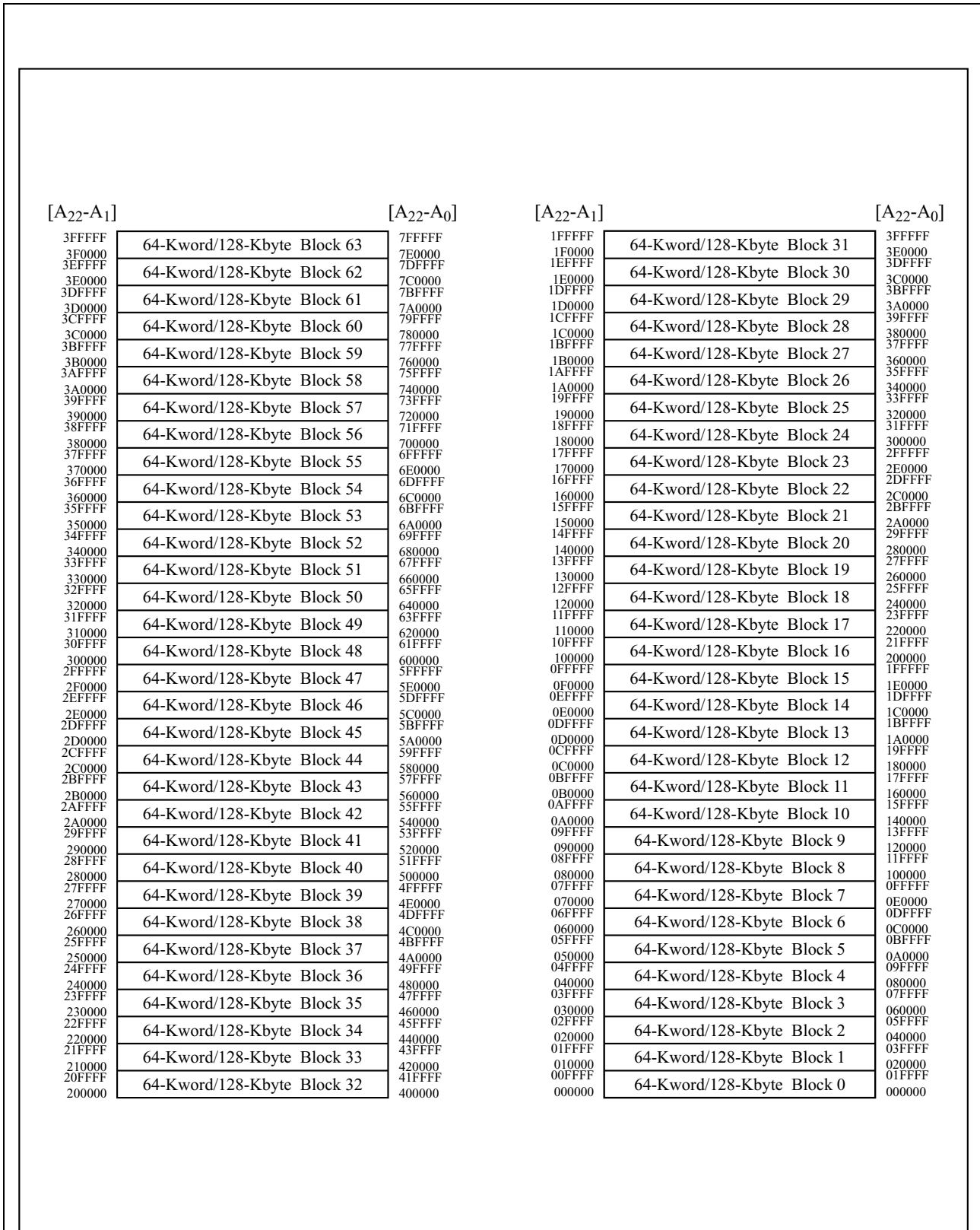
Figure 2. Memory Map
