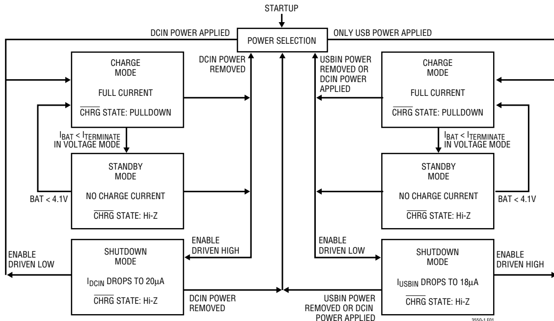
Figure 1. LTC3550-1 State Diagram of a Charge Cycle
