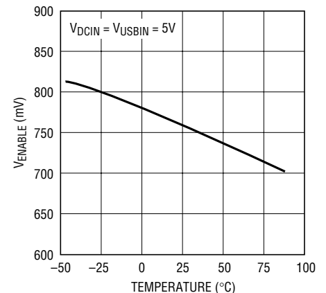
ENABLE Pin Threshold Voltage (On-to-Off) vs Temperature
