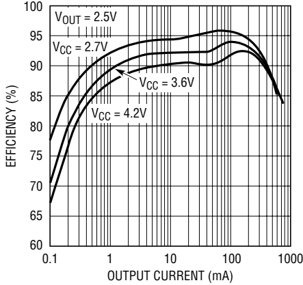
Buck Regulator Efficiency vs Output Current
