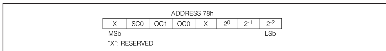
Figure 20. Overcurrent and Short-Circuit Threshold Bits Format
