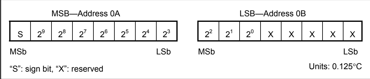
Figure 5. TEMPERATURE REGISTER FORMAT
