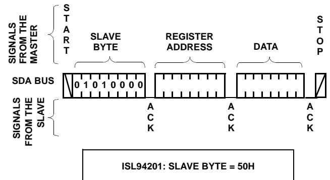
FIGURE 9. WRITE SEQUENCE
