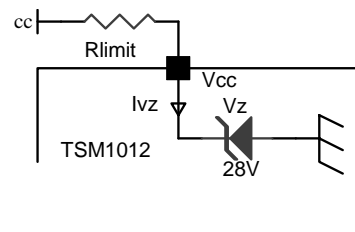
Figure 4 : Clamp voltage
