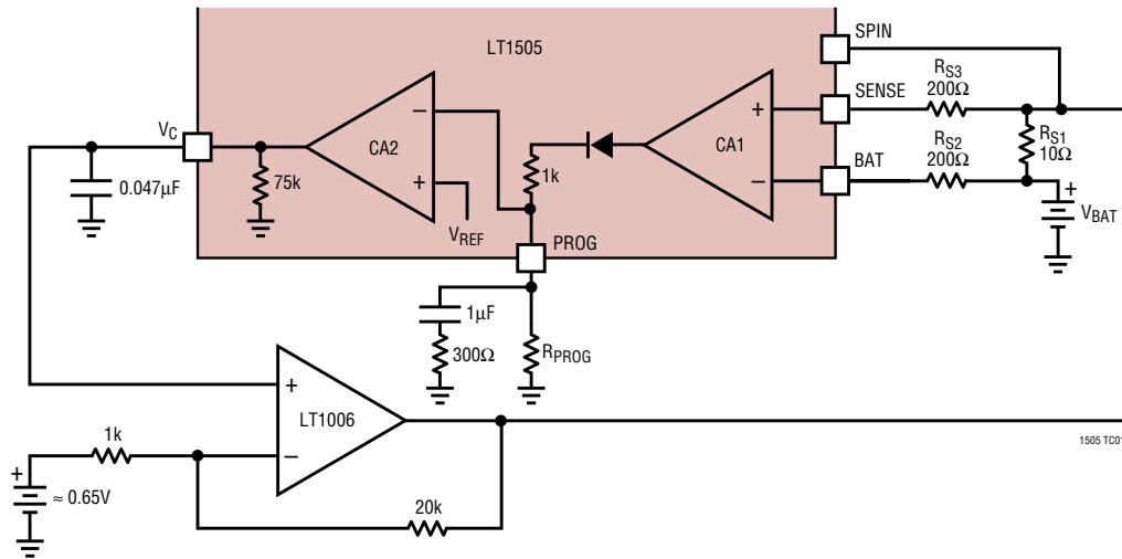
Test Circuit 2
