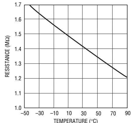
EN_CHRG Pin Pulldown Resistance vs Temperature
