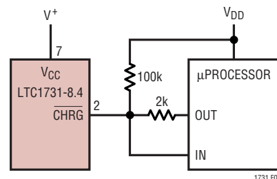
Figure 1. Microprocessor Interface
