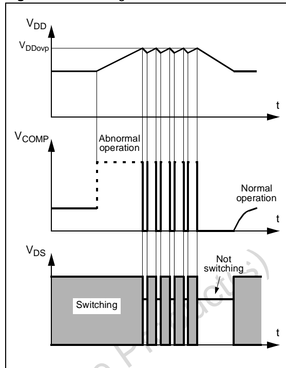
Figure 7: Overvoltage Event
