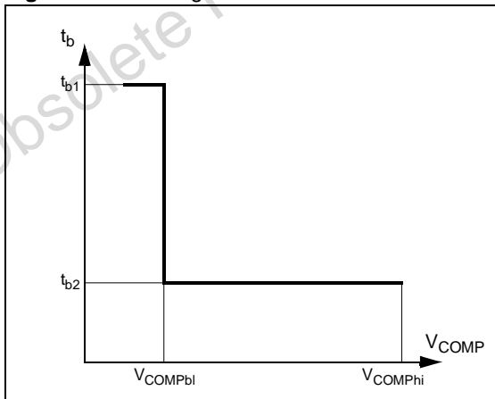
Figure 11: Blanking Time
