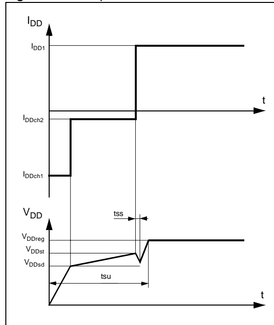
Figure 17: Startup Waveforms
