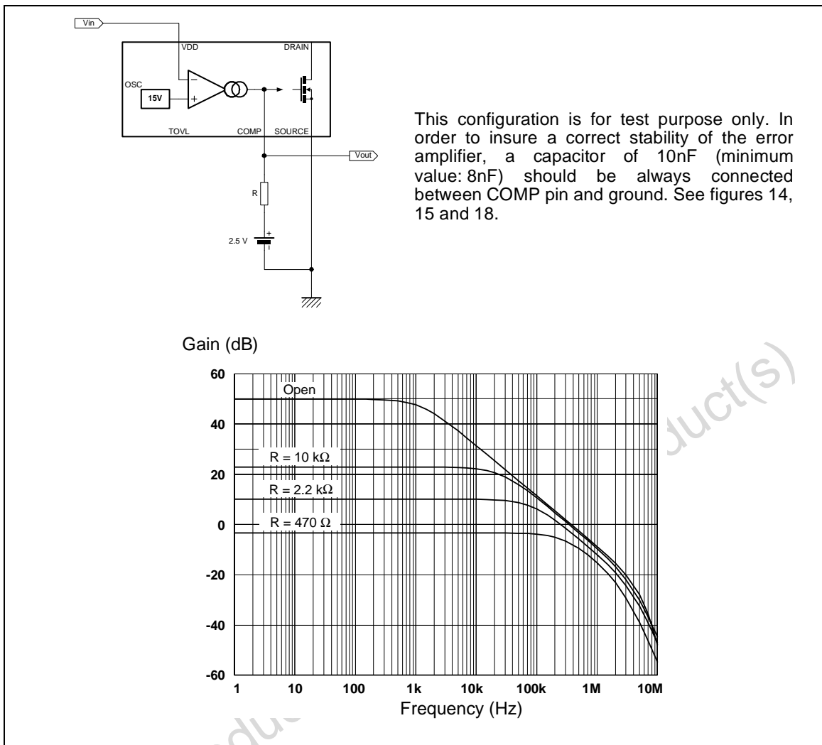
Figure 10: Error Amplifier Transfer Function
