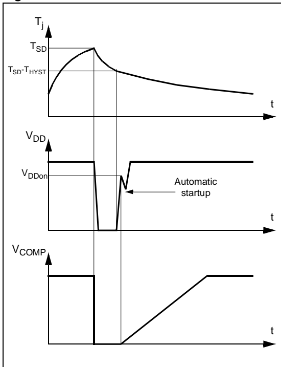
Figure 5: Thermal Shutdown
