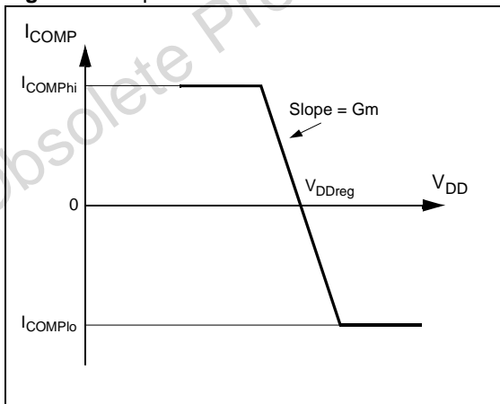
Figure 3: Output Characteristics
