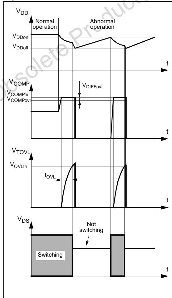
Figure 4: Overload event
