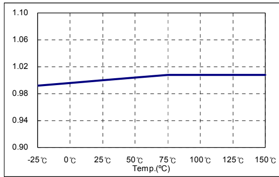
Figure 21. Normal Mode Sync. Low Threshold Voltage
