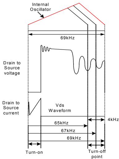
Figure 10. Frequency Modulation Waveform
