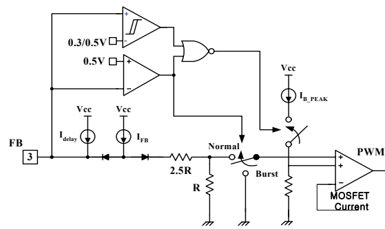
Figure 8. Circuit for Burst operation
