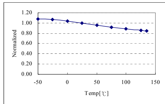
J-FET Start up current (Istr)
