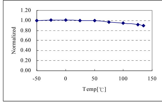
Peak current limit (Iover)
