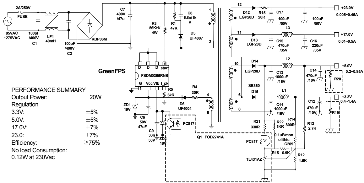
Figure15. 20W multiple power supply using FSDM0365RNB
