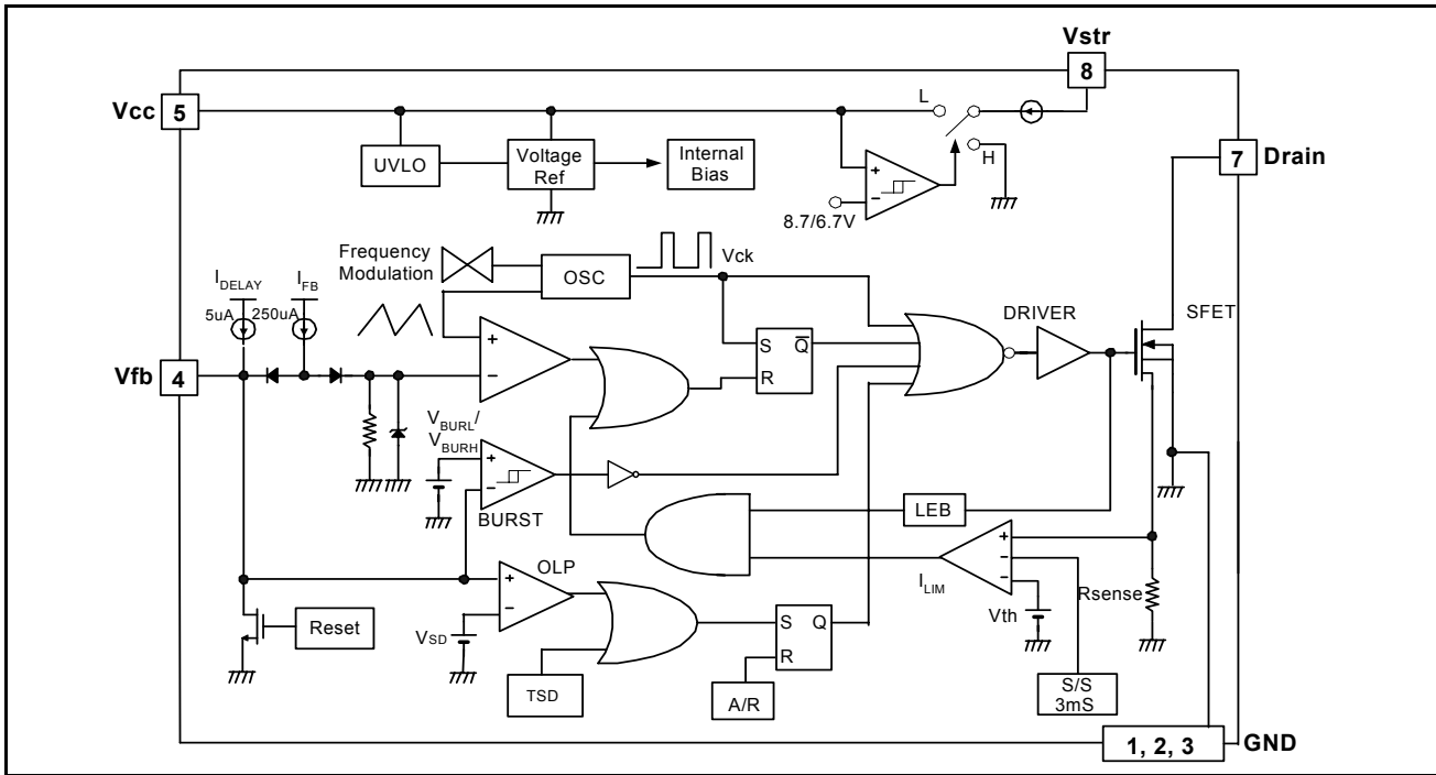
Figure 3. Functional Block Diagram of FSD210B
