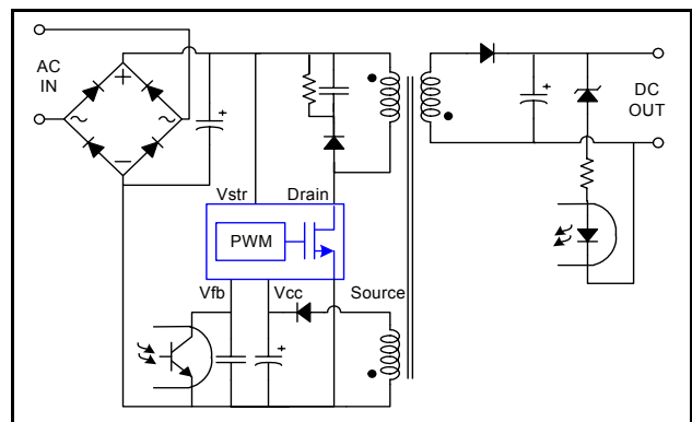
Figure 1. Typical Flyback Application for FSD210B
