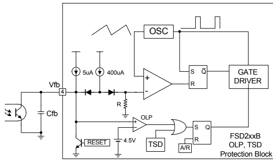
Figure 9. Protection Block
