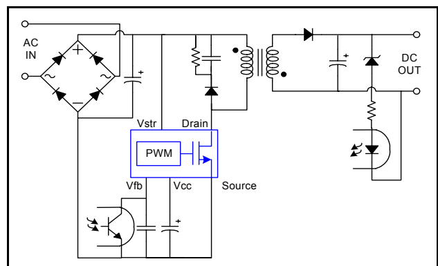
Figure 2. Typical Flyback Application for FSD200B
