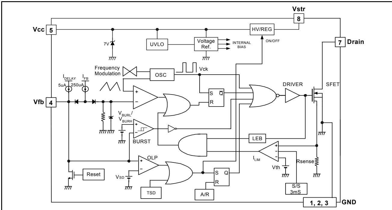
Figure 4. Functional Block Diagram of FSD200B
