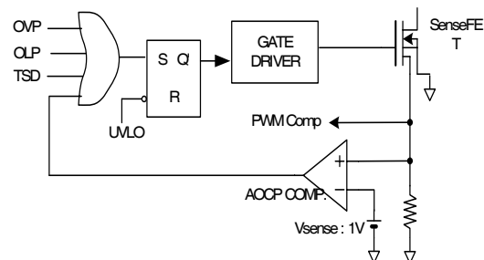
Figure 25. AOCP block
