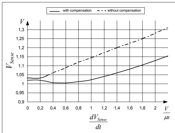
Figure 13 Overcurrent Shutdown
