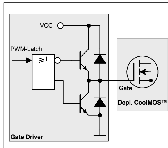
Figure 8 Gate Driver
