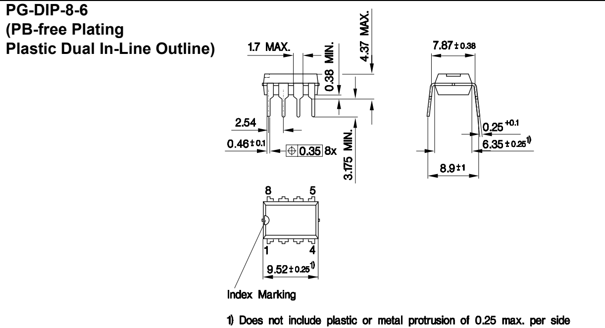
Figure 23 PG-DIP-8-6 (PB-free Plating Plastic Dual In-Line Outline)
