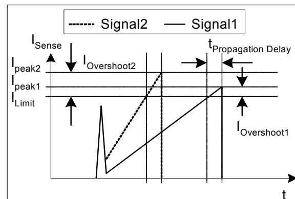
Figure 12 Current Limiting
