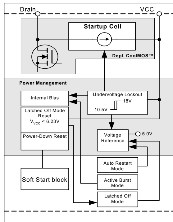
Figure 3 Power Management
