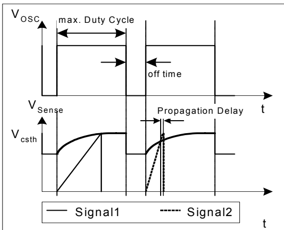
Figure 14 Dynamic Voltage Threshold V_{csth}
