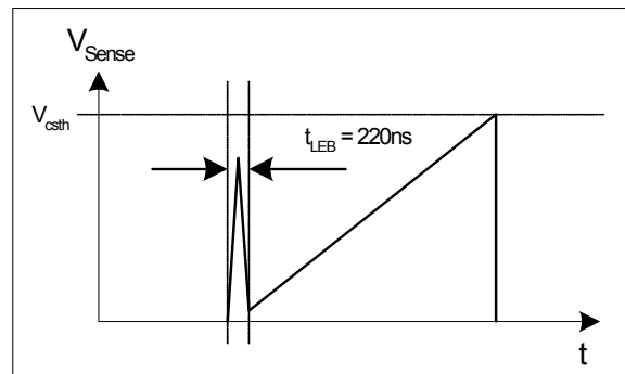
Figure 11 Leading Edge Blanking
