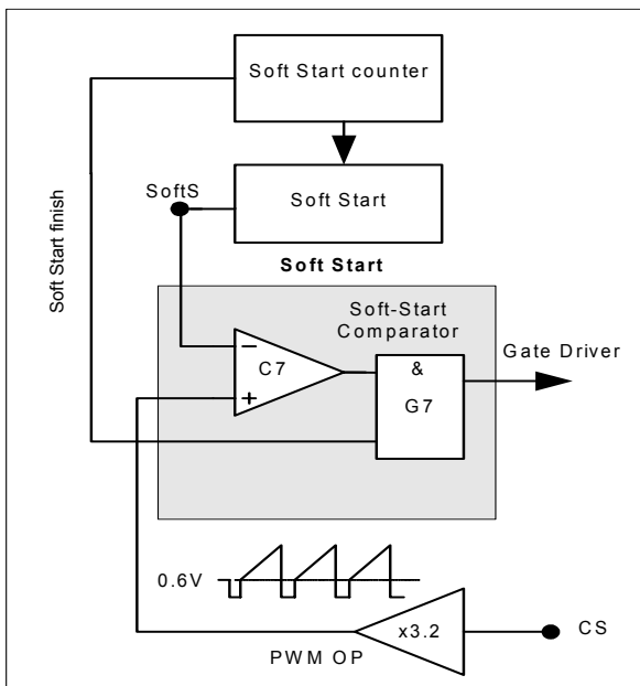
Figure 4 Soft Start
