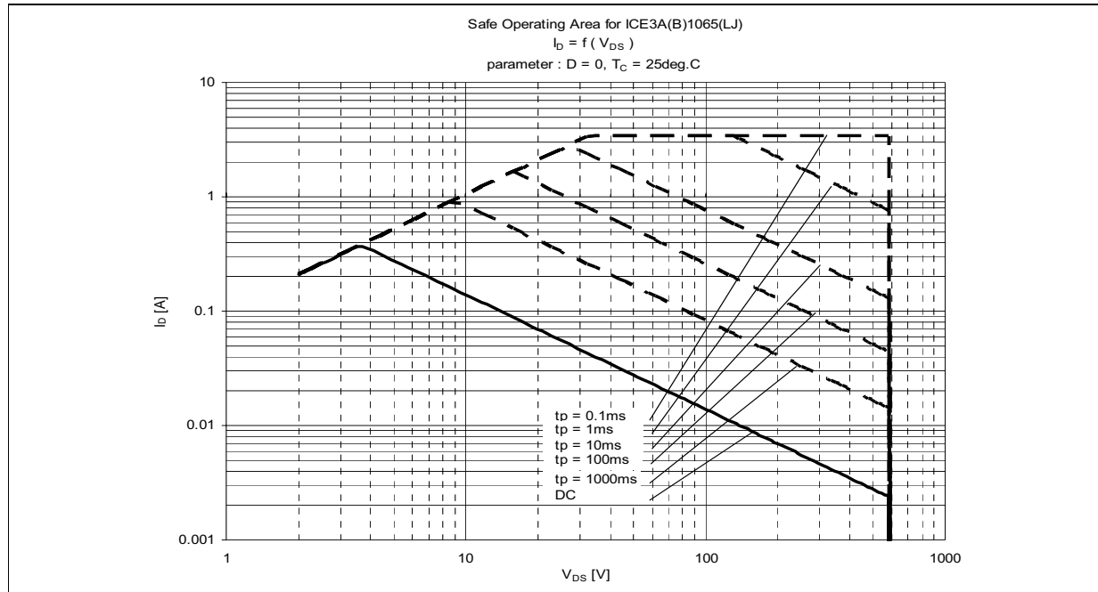
Figure 21 Safe Operating area ( SOA ) curve
