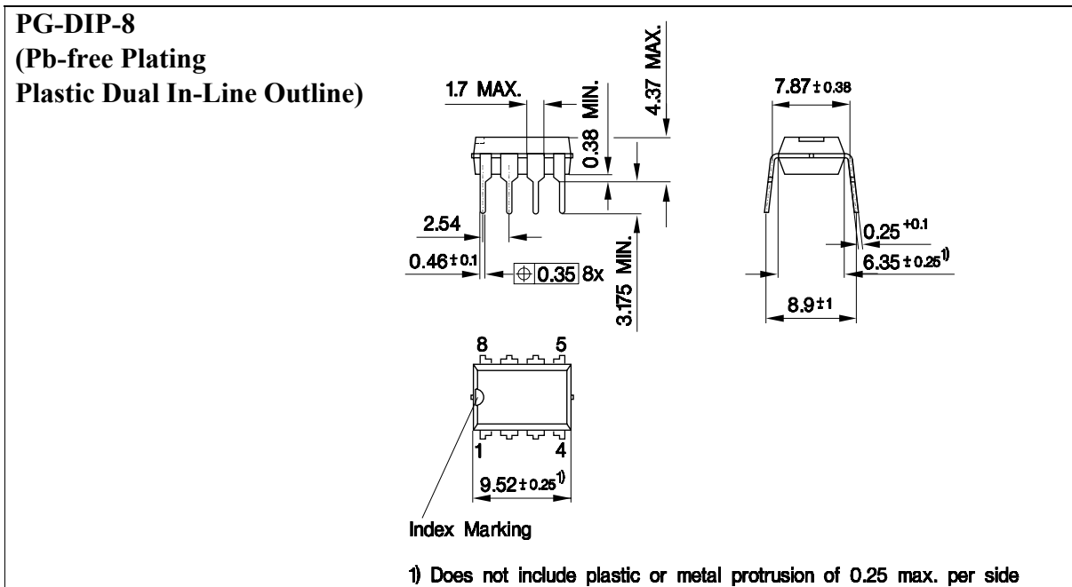
Figure 19 PG-DIP-8 (Pb-free Plating Plastic Dual In-Line Outline)
