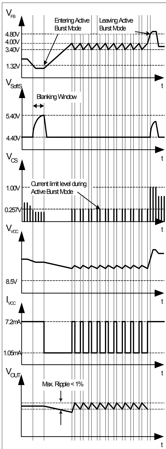
Figure 17 Signals in Active Burst Mode
