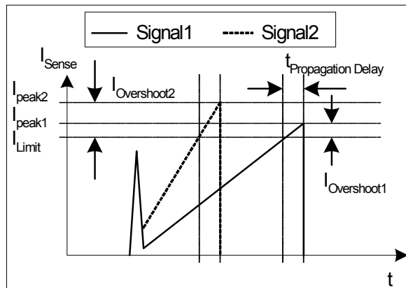
Figure 12 Current Limiting
