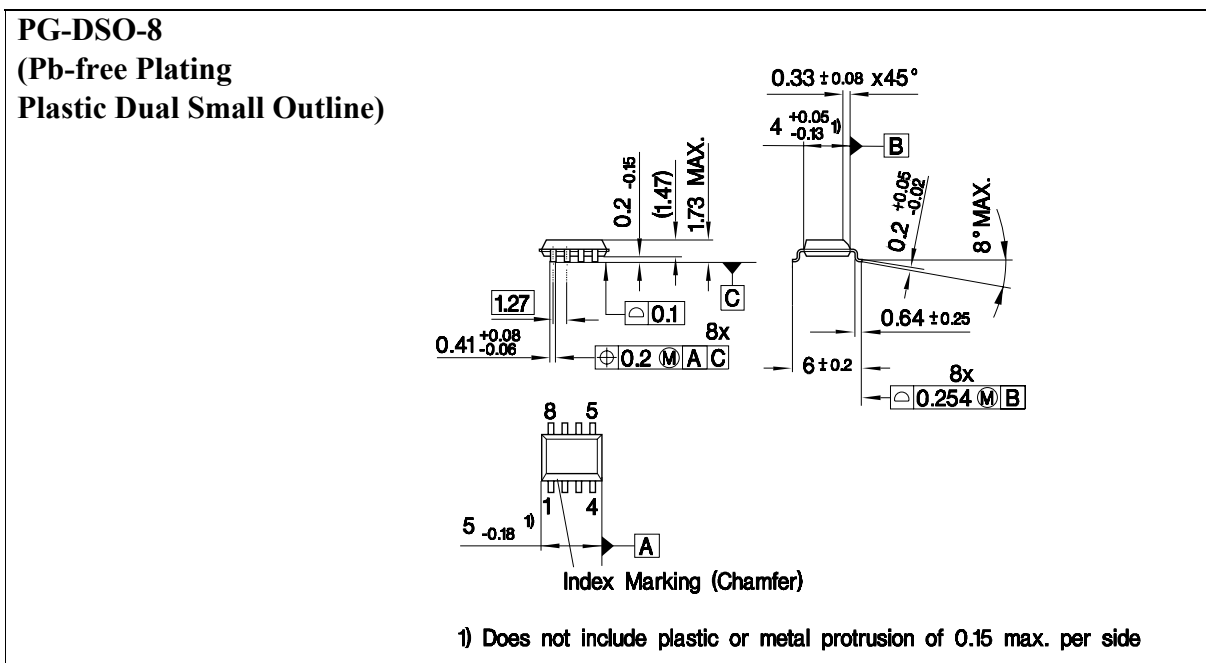
Figure 20 GP-DSO-8 (Pb-free Plating Plastic Dual Small Outline)
