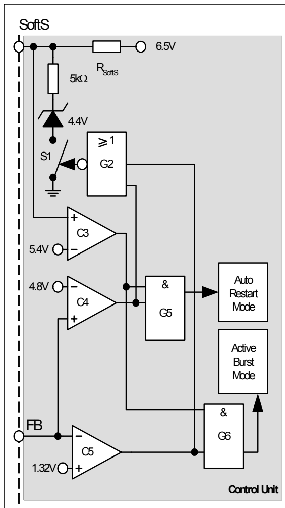
Figure 15 Adjustable Blanking Window
