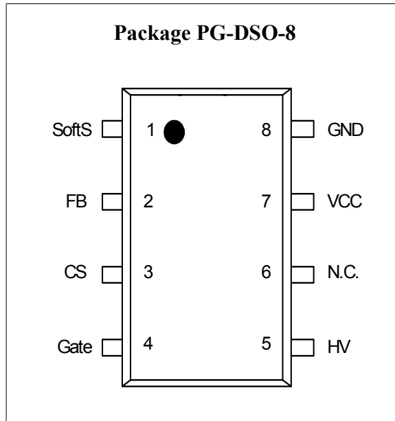
Figure 2 Pin Configuration PG-DSO-8(top view)
