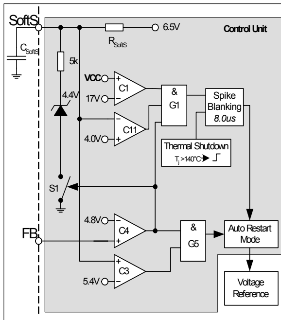
Figure 18 Auto Restart Mode
