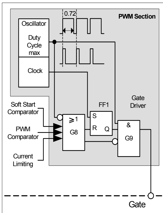
Figure 7 PWM Section
