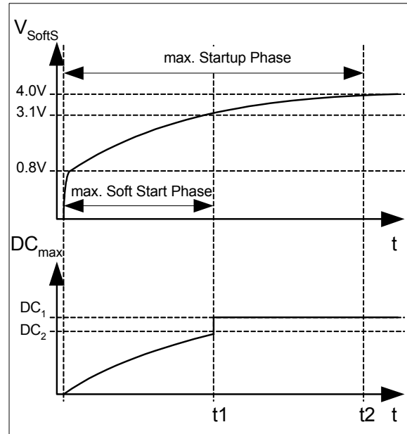
Figure 5 Startup Phase
