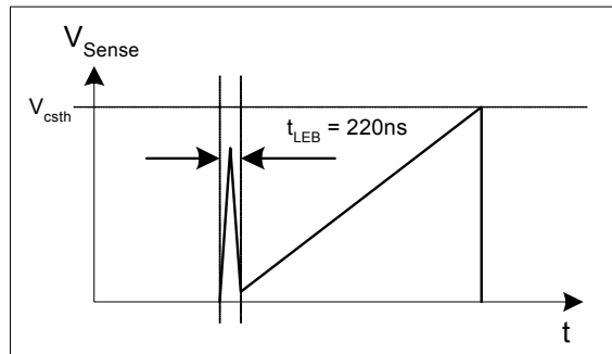
Figure 9 Leading Edge Blanking
