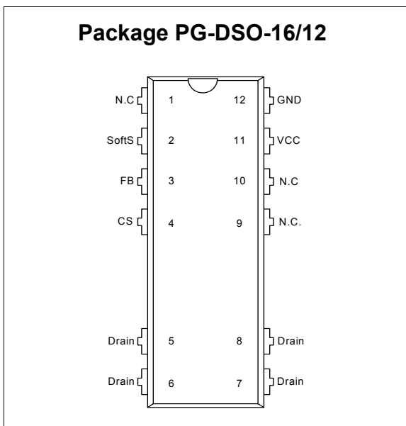
Figure 1 Pin Configuration PG-DSO-16/12
