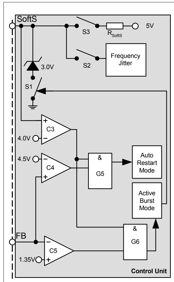
Figure 13 Adjustable Blanking Window
