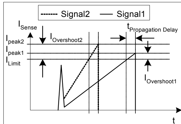
Figure 10 Current Limiting
