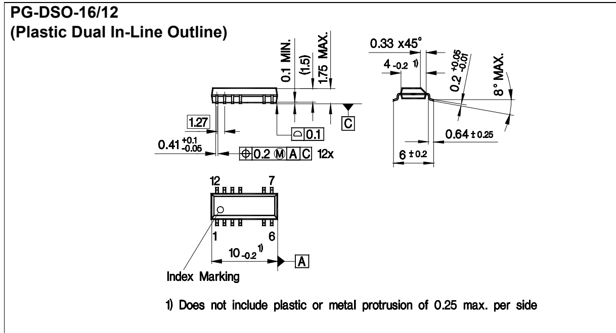
Figure 18 PG-DSO-16/12
