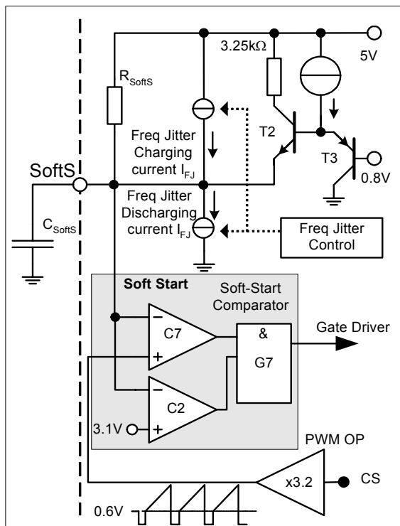
Figure 4 Soft Start
