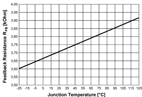
Figure 38 Feedback Resistance R_{FB} vs. T_j
