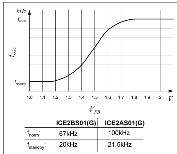
Figure 12 Frequency Dependence
