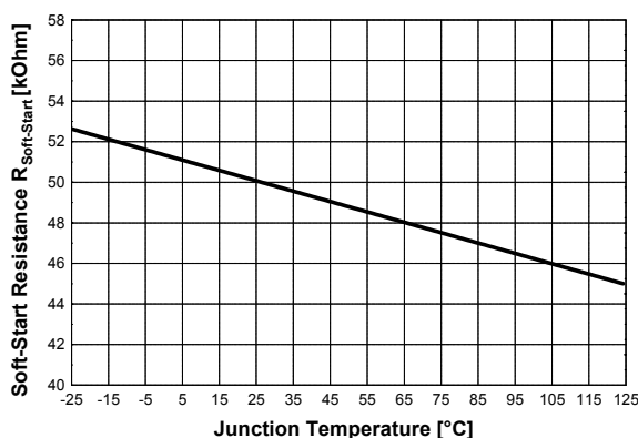
Figure 39 Soft-Start Resistance R_{Soft-Start} vs. T_j
