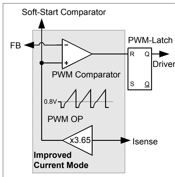
Figure 4 Current Mode
