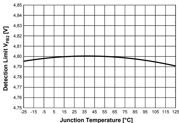
Figure 40 Detection Limit V_{FB2} vs. T_j
