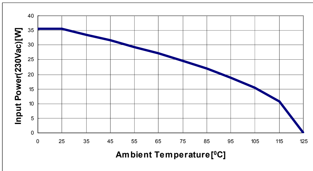
Figure 13 Input Power curve V_{in}=230\text{Vac}; P_{in}=f(T_a)
