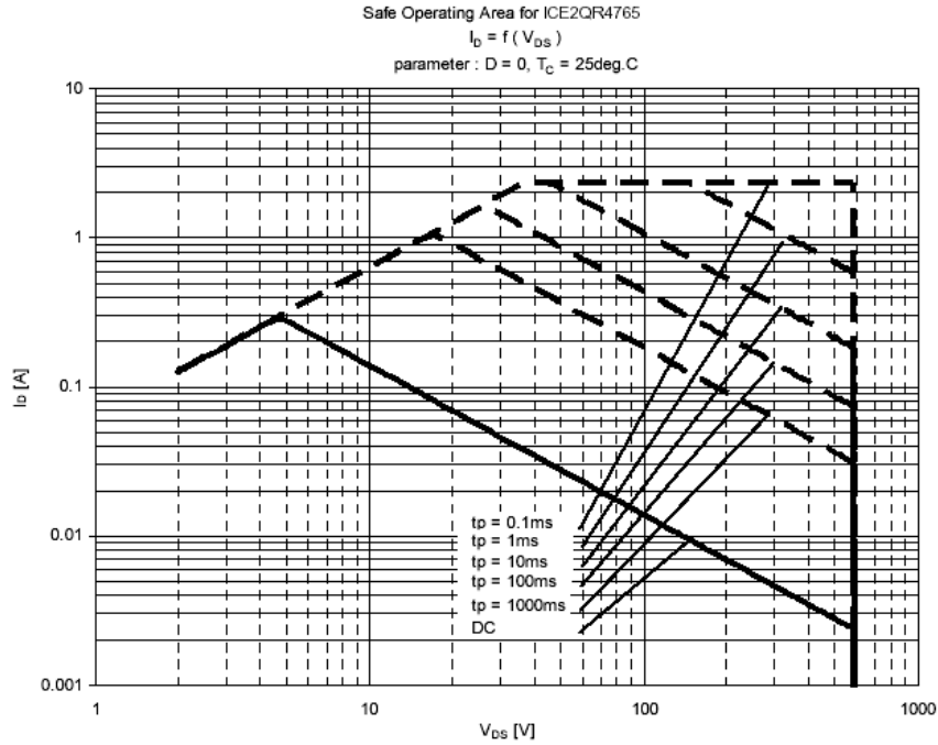
Figure 9 Safe Operating Area(SOA) curve for ICE2QR4765
