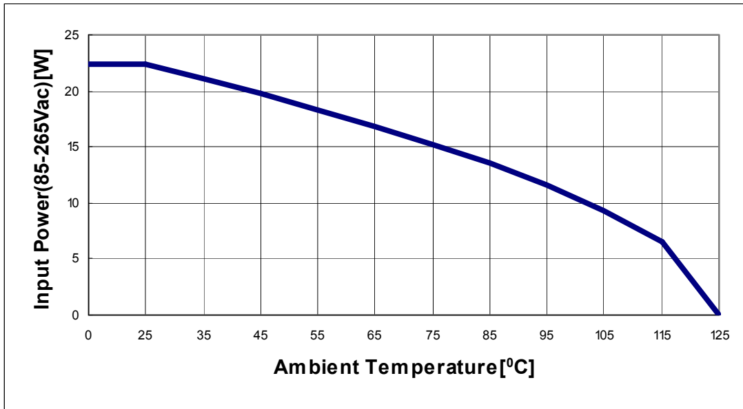
Figure 12 Input Power curve V_{in}=85\sim 265\text{Vac}; P_{in}=f(T_a)
