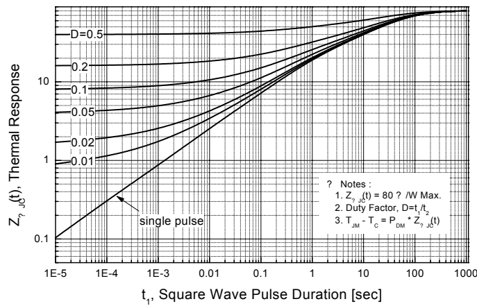
Figure 11. Thermal Response
